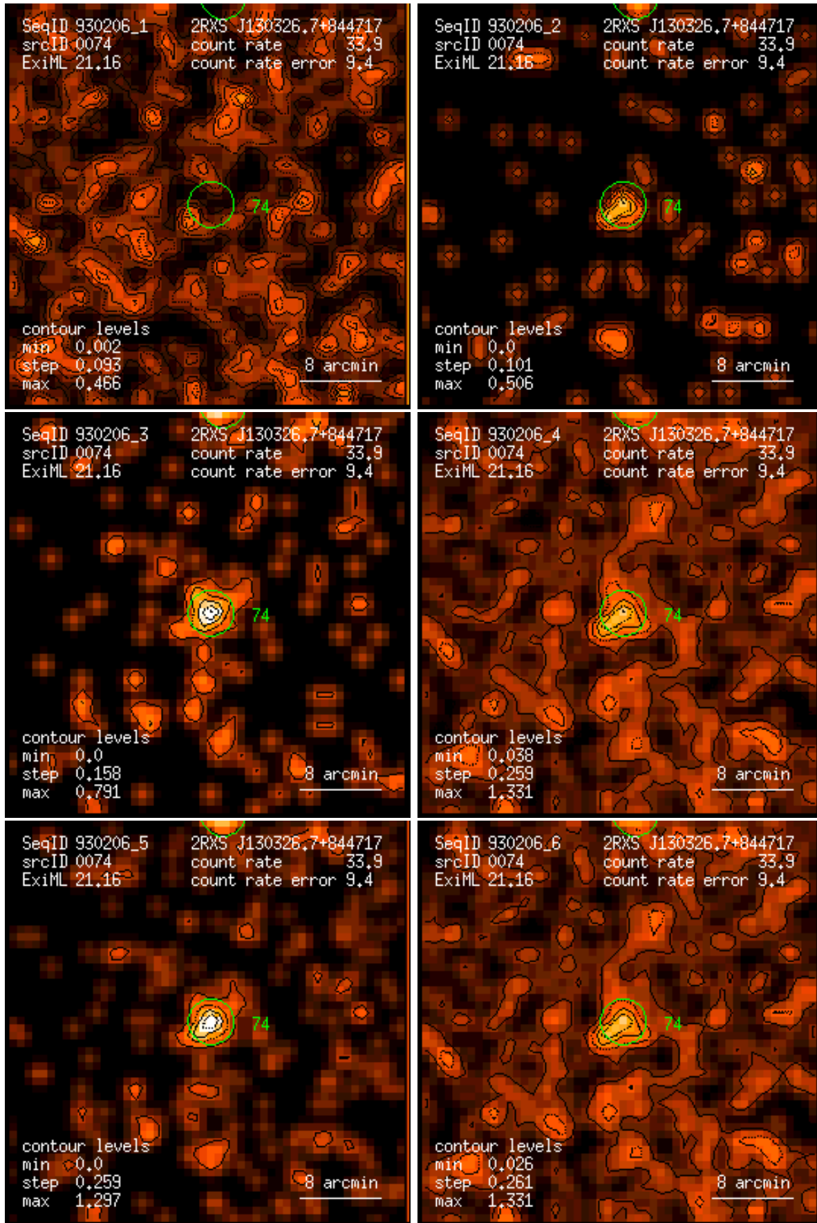
Figure 74: RASS 930206: detection 0074: band rate images, Gaussian filter: (1) PSPC channels 11 – 41, (2) 52 – 90, (3) 91 – 201, (4) 11 – 235, (5) 52 – 201, (6) 11 – 201. Broad band rates in counts/ks. Band rate contour levels in counts/ks/arcmin 2 .
