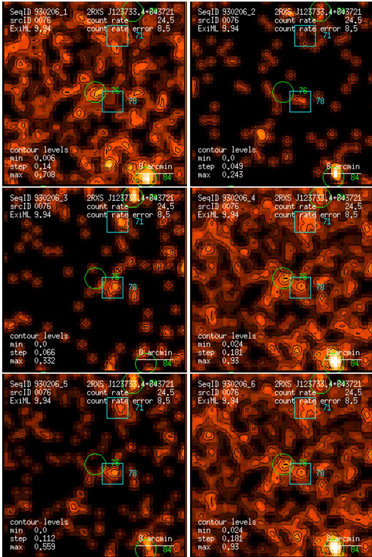
Figure 76: RASS 930206: detection 0076: band rate images, Gaussian filter: (1) PSPC channels 11 – 41, (2) 52 – 90, (3) 91 – 201, (4) 11 – 235, (5) 52 – 201, (6) 11 – 201. Broad band rates in counts/ks. Band rate contour levels in counts/ks/arcmin 2 .
