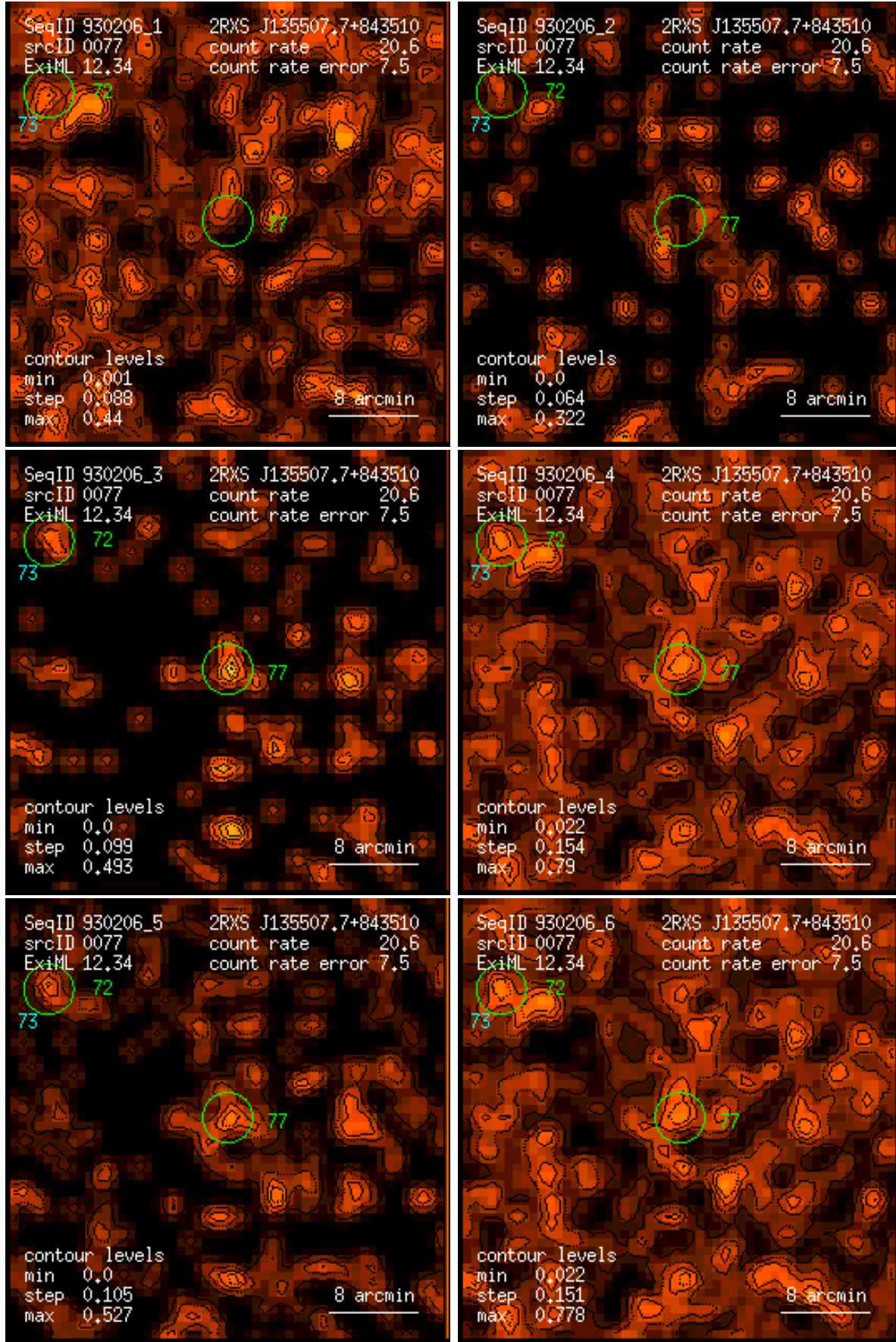
Figure 77: RASS 930206: detection 0077: band rate images, Gaussian filter: (1) PSPC channels 11 – 41, (2) 52 – 90, (3) 91 – 201, (4) 11 – 235, (5) 52 – 201, (6) 11 – 201. Broad band rates in counts/ks. Band rate contour levels in counts/ks/arcmin 2 .
