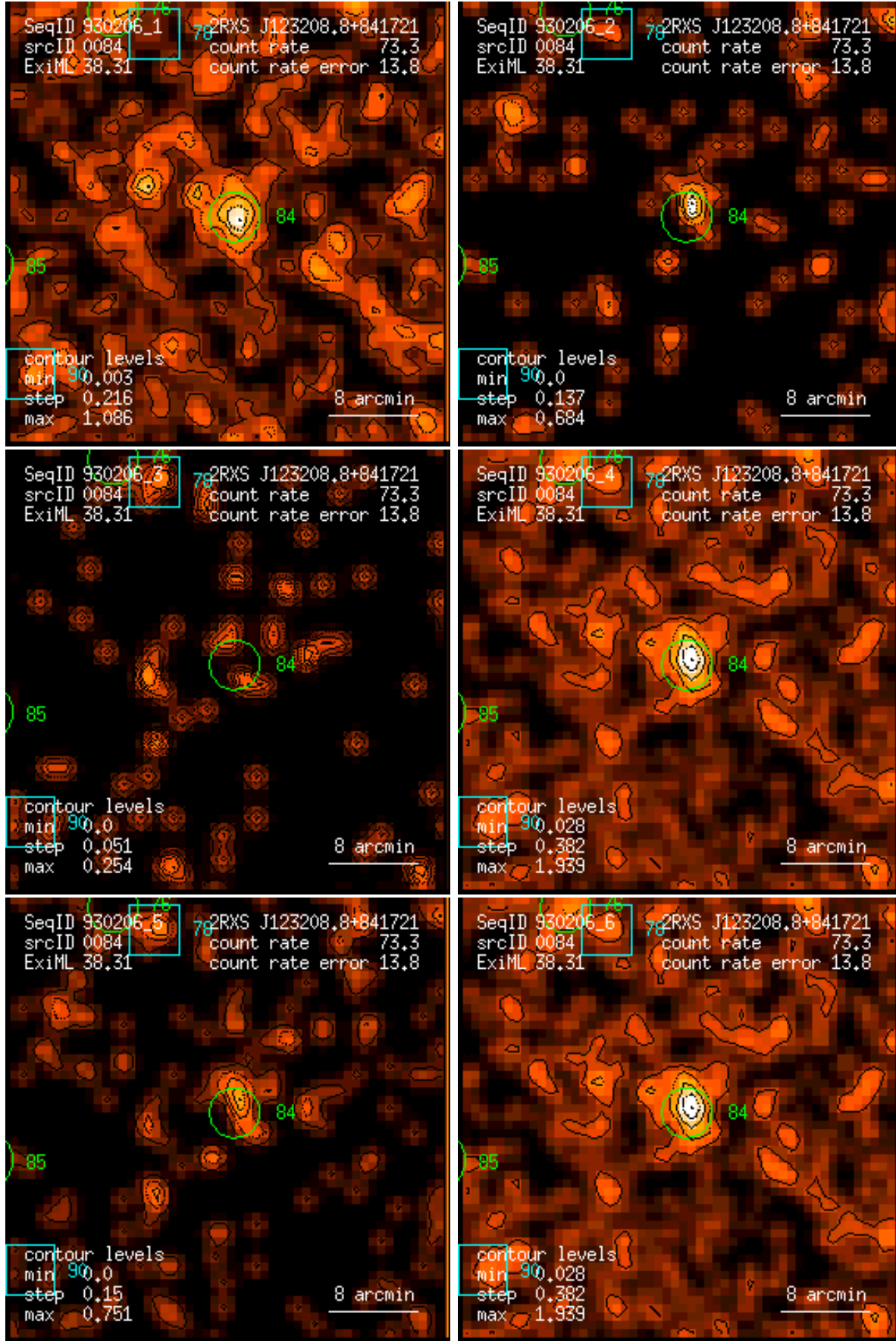
Figure 84: RASS 930206: detection 0084: band rate images, Gaussian filter: (1) PSPC channels 11 – 41, (2) 52 – 90, (3) 91 – 201, (4) 11 – 235, (5) 52 – 201, (6) 11 – 201. Broad band rates in counts/ks. Band rate contour levels in counts/ks/arcmin 2 .
