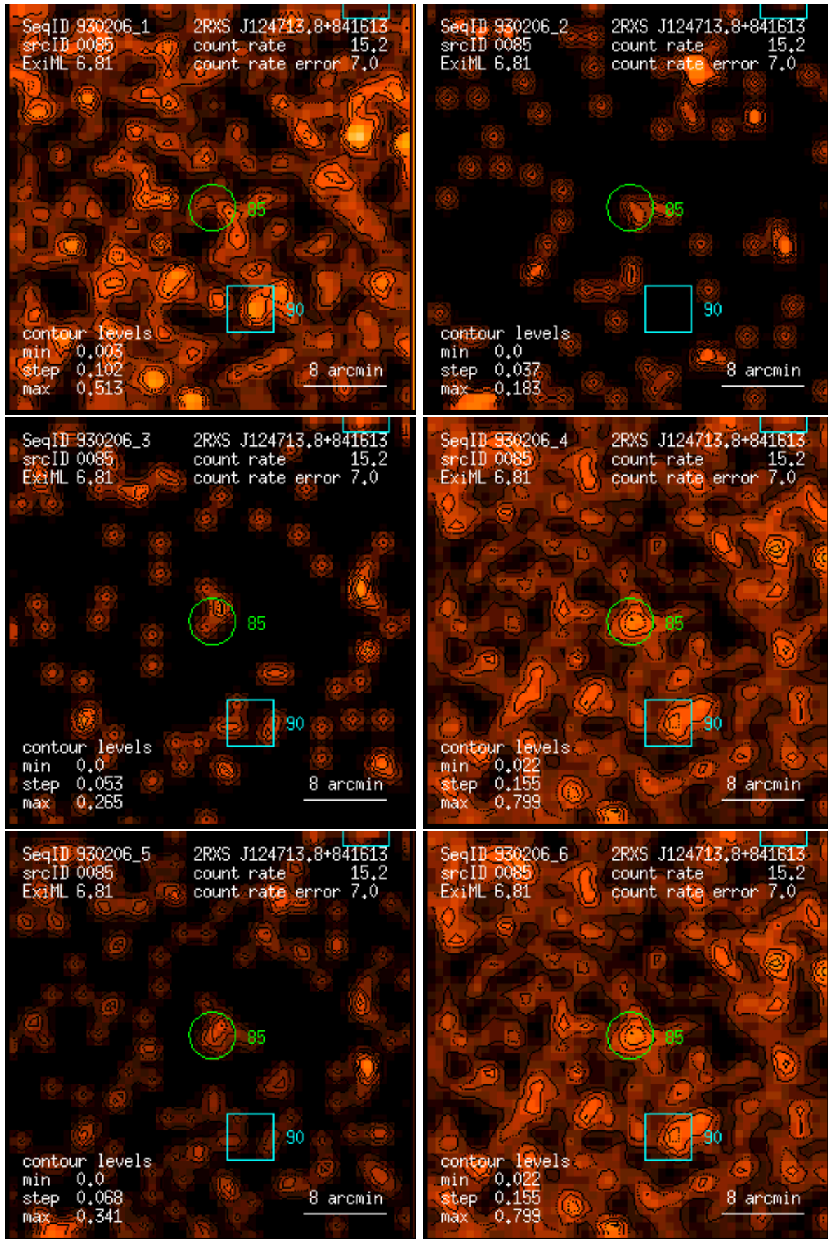
Figure 85: RASS 930206: detection 0085: band rate images, Gaussian filter: (1) PSPC channels 11 – 41, (2) 52 – 90, (3) 91 – 201, (4) 11 – 235, (5) 52 – 201, (6) 11 – 201. Broad band rates in counts/ks. Band rate contour levels in counts/ks/arcmin 2 .
