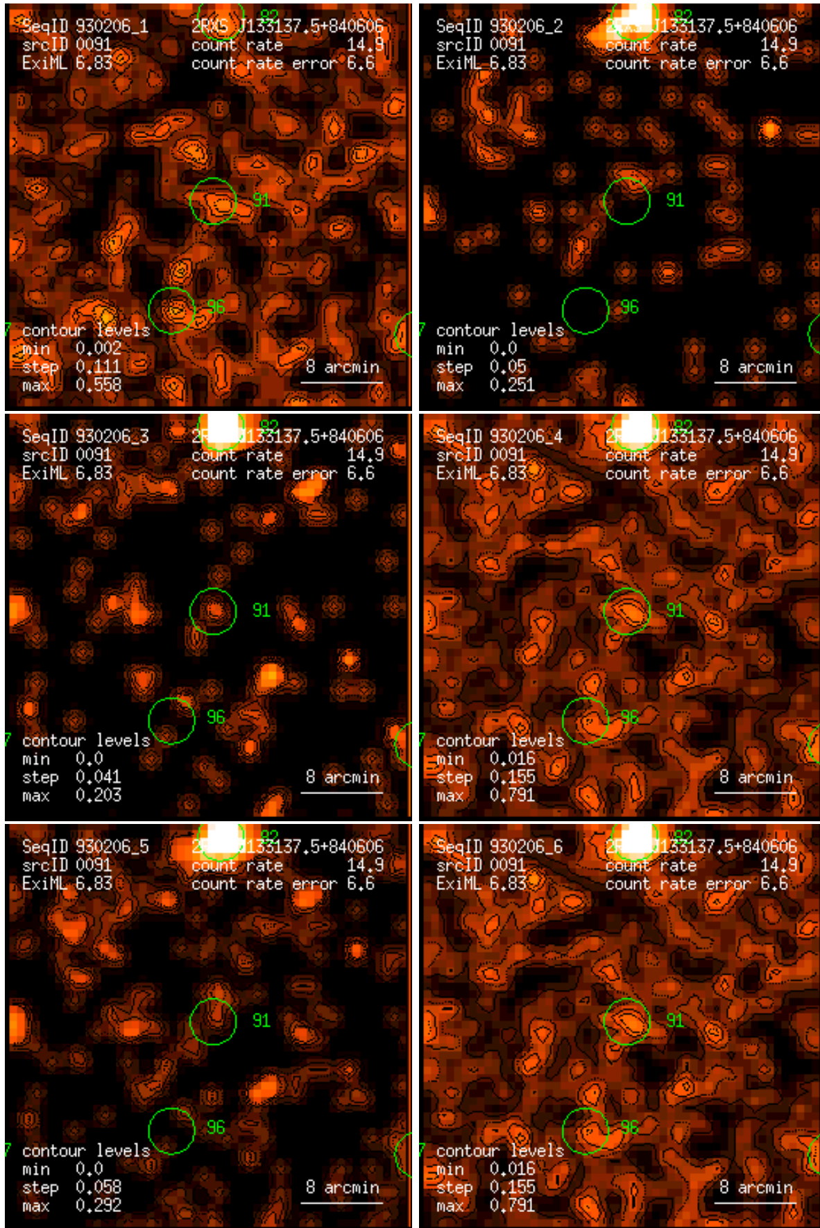
Figure 91: RASS 930206: detection 0091: band rate images, Gaussian filter: (1) PSPC channels 11 – 41, (2) 52 – 90, (3) 91 – 201, (4) 11 – 235, (5) 52 – 201, (6) 11 – 201. Broad band rates in counts/ks. Band rate contour levels in counts/ks/arcmin 2 .
