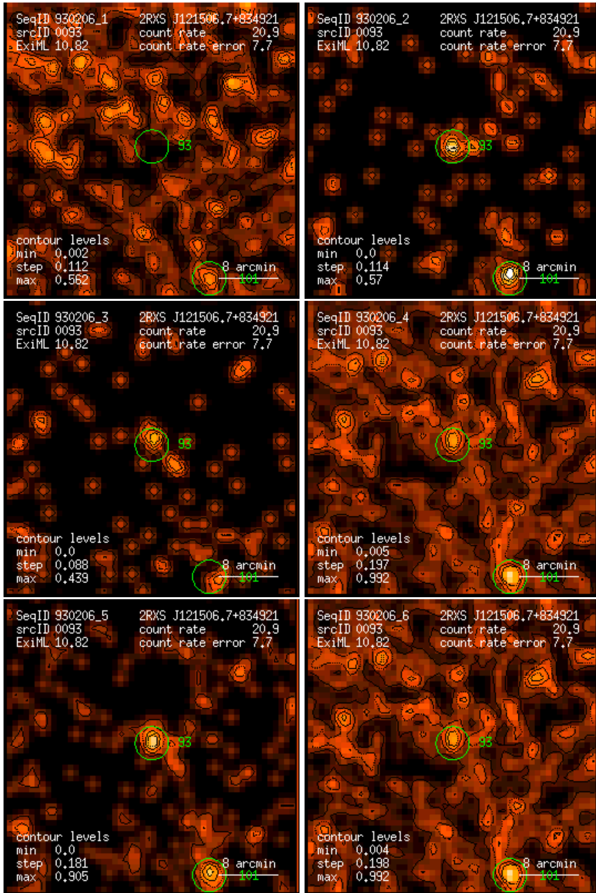
Figure 93: RASS 930206: detection 0093: band rate images, Gaussian filter: (1) PSPC channels 11 – 41, (2) 52 – 90, (3) 91 – 201, (4) 11 – 235, (5) 52 – 201, (6) 11 – 201. Broad band rates in counts/ks. Band rate contour levels in counts/ks/arcmin 2 .
