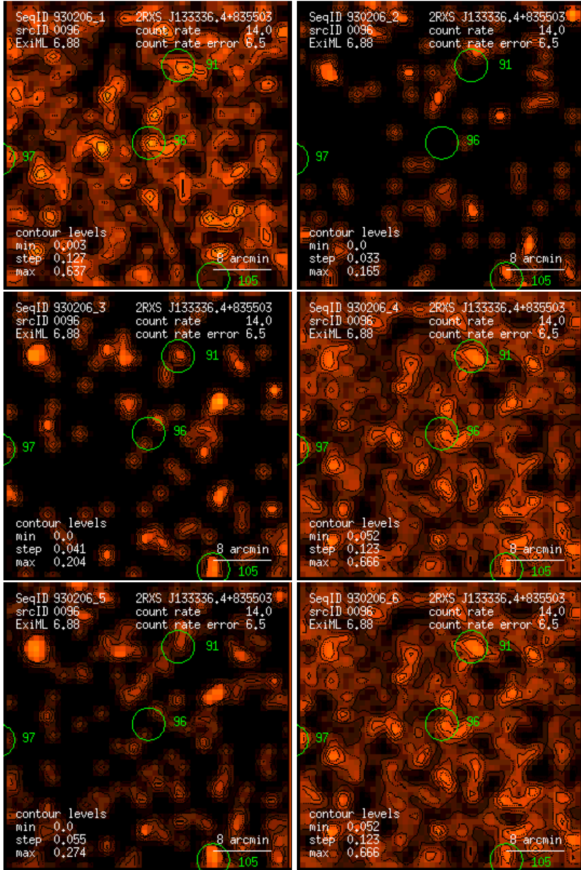
Figure 96: RASS 930206: detection 0096: band rate images, Gaussian filter: (1) PSPC channels 11 – 41, (2) 52 – 90, (3) 91 – 201, (4) 11 – 235, (5) 52 – 201, (6) 11 – 201. Broad band rates in counts/ks. Band rate contour levels in counts/ks/arcmin 2 .
