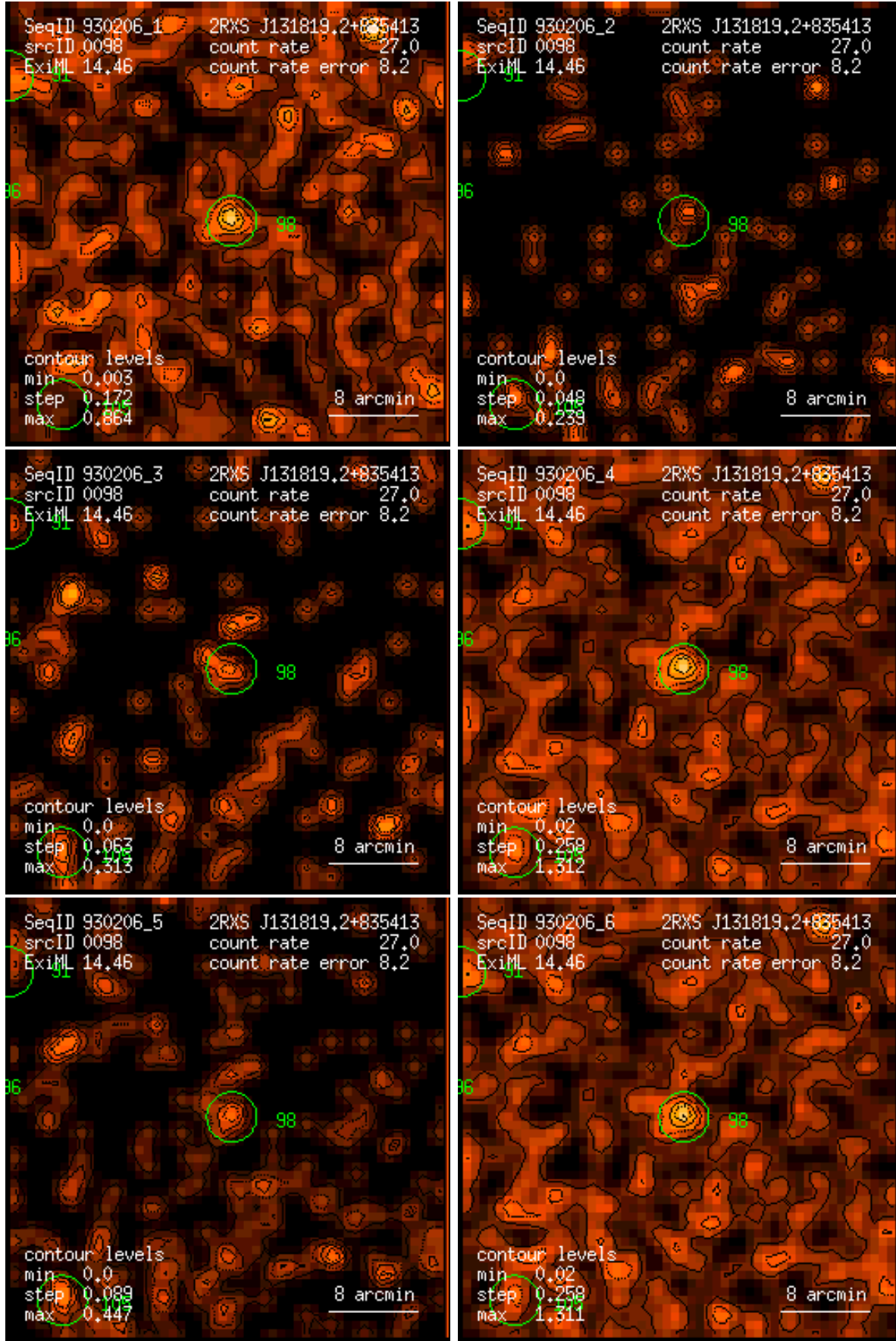
Figure 98: RASS 930206: detection 0098: band rate images, Gaussian filter: (1) PSPC channels 11 – 41, (2) 52 – 90, (3) 91 – 201, (4) 11 – 235, (5) 52 – 201, (6) 11 – 201. Broad band rates in counts/ks. Band rate contour levels in counts/ks/arcmin 2 .
