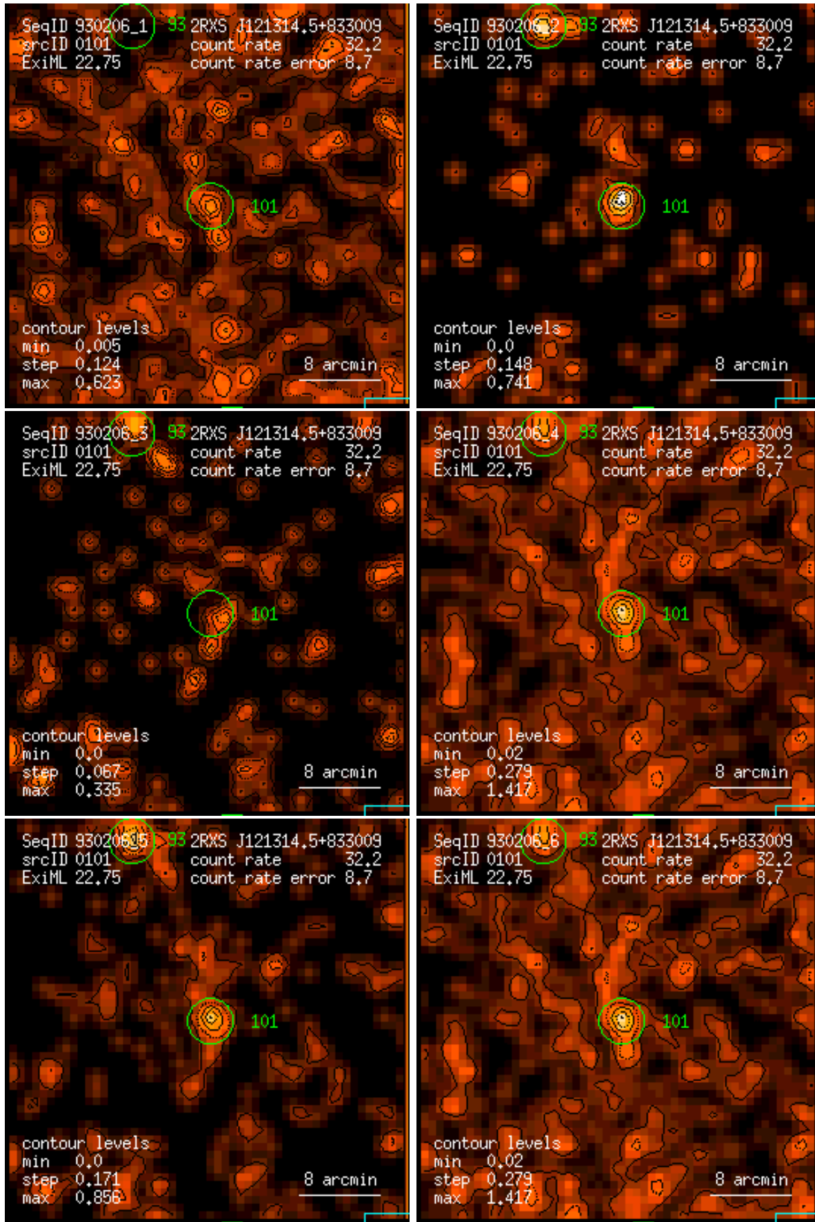
Figure 101: RASS 930206: detection 0101: band rate images, Gaussian filter: (1) PSPC channels 11 – 41, (2) 52 – 90, (3) 91 – 201, (4) 11 – 235, (5) 52 – 201, (6) 11 – 201. Broad band rates in counts/ks. Band rate contour levels in counts/ks/arcmin 2 .
