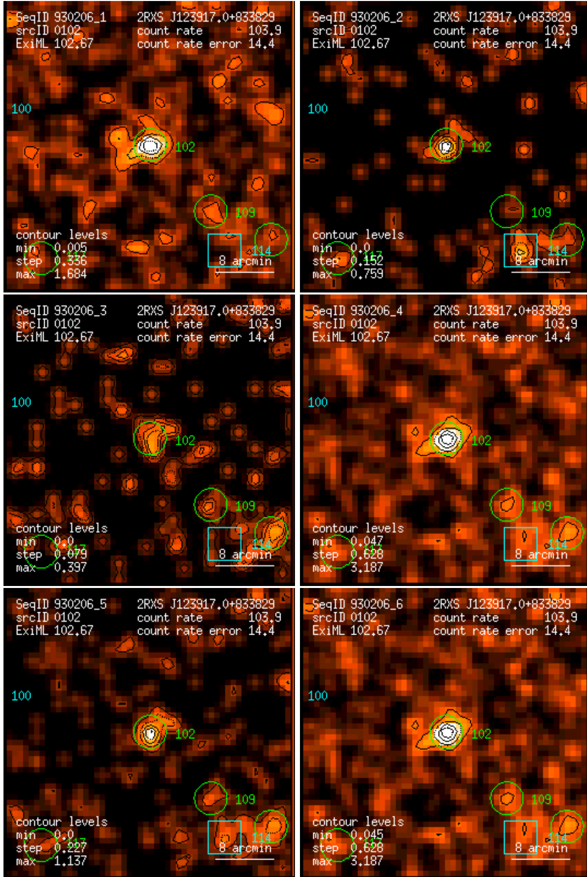
Figure 102: RASS 930206: detection 0102: band rate images, Gaussian filter: (1) PSPC channels 11 – 41, (2) 52 – 90, (3) 91 – 201, (4) 11 – 235, (5) 52 – 201, (6) 11 – 201. Broad band rates in counts/ks. Band rate contour levels in counts/ks/arcmin 2 .
