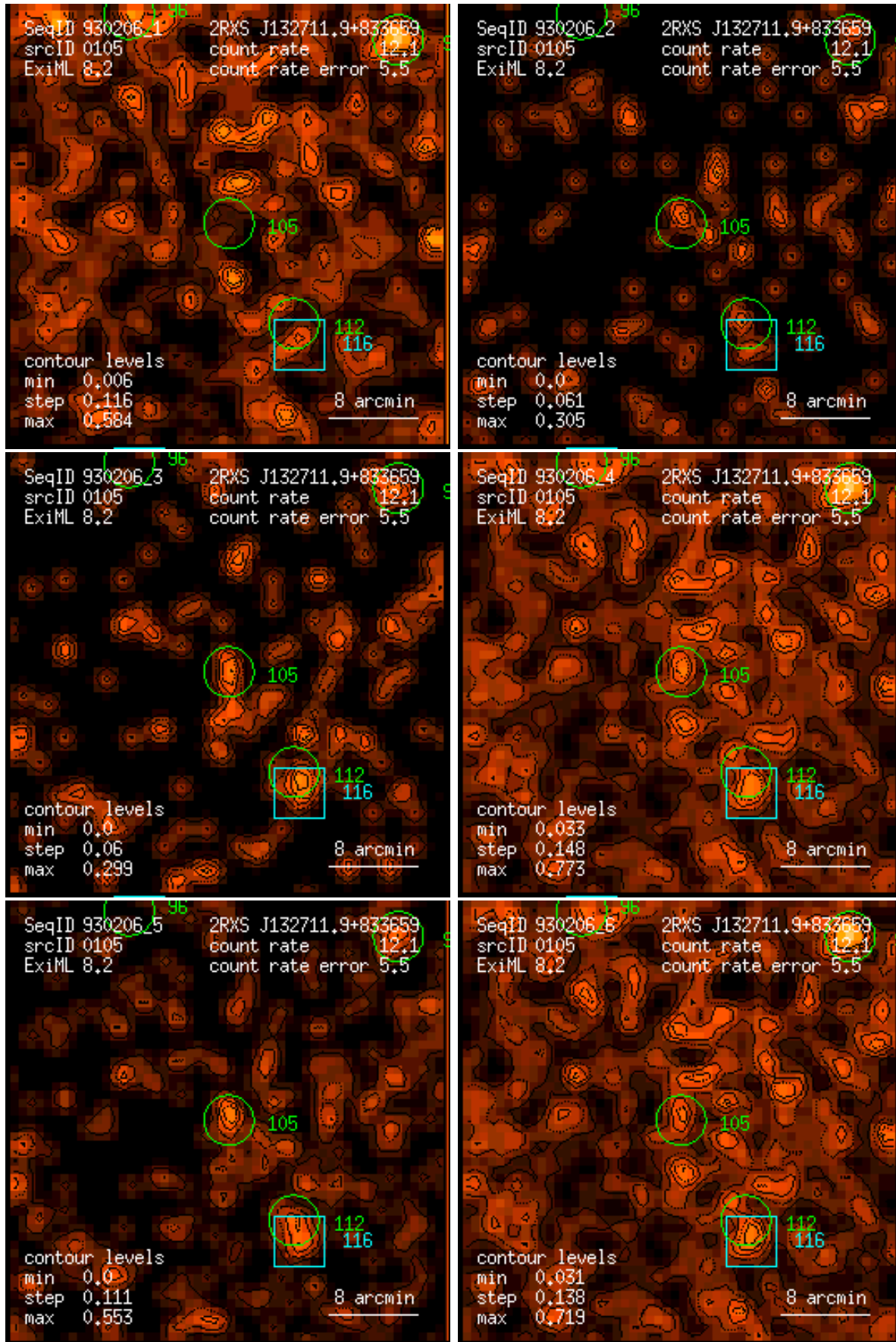
Figure 105: RASS 930206: detection 0105: band rate images, Gaussian filter: (1) PSPC channels 11 – 41, (2) 52 – 90, (3) 91 – 201, (4) 11 – 235, (5) 52 – 201, (6) 11 – 201. Broad band rates in counts/ks. Band rate contour levels in counts/ks/arcmin 2 .
