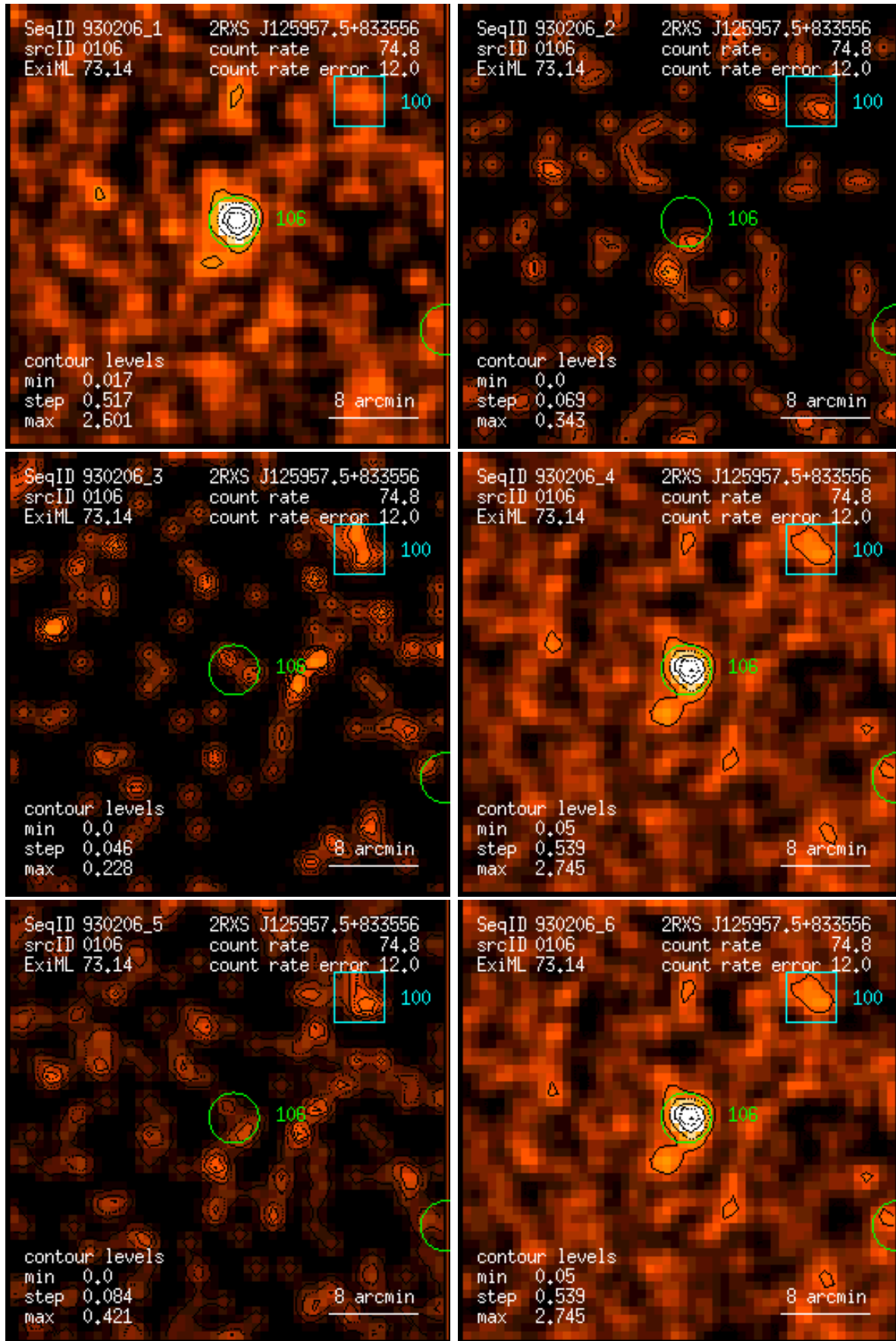
Figure 106: RASS 930206: detection 0106: band rate images, Gaussian filter: (1) PSPC channels 11 – 41, (2) 52 – 90, (3) 91 – 201, (4) 11 – 235, (5) 52 – 201, (6) 11 – 201. Broad band rates in counts/ks. Band rate contour levels in counts/ks/arcmin 2 .
