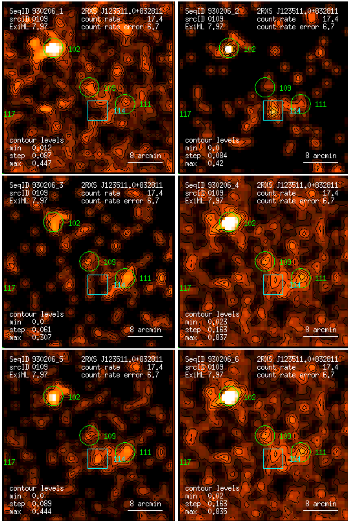
Figure 109: RASS 930206: detection 0109: band rate images, Gaussian filter: (1) PSPC channels 11 – 41, (2) 52 – 90, (3) 91 – 201, (4) 11 – 235, (5) 52 – 201, (6) 11 – 201. Broad band rates in counts/ks. Band rate contour levels in counts/ks/arcmin 2 .
