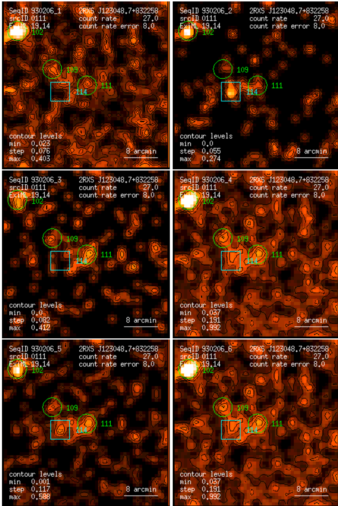
Figure 111: RASS 930206: detection 0111: band rate images, Gaussian filter: (1) PSPC channels 11 – 41, (2) 52 – 90, (3) 91 – 201, (4) 11 – 235, (5) 52 – 201, (6) 11 – 201. Broad band rates in counts/ks. Band rate contour levels in counts/ks/arcmin 2 .
