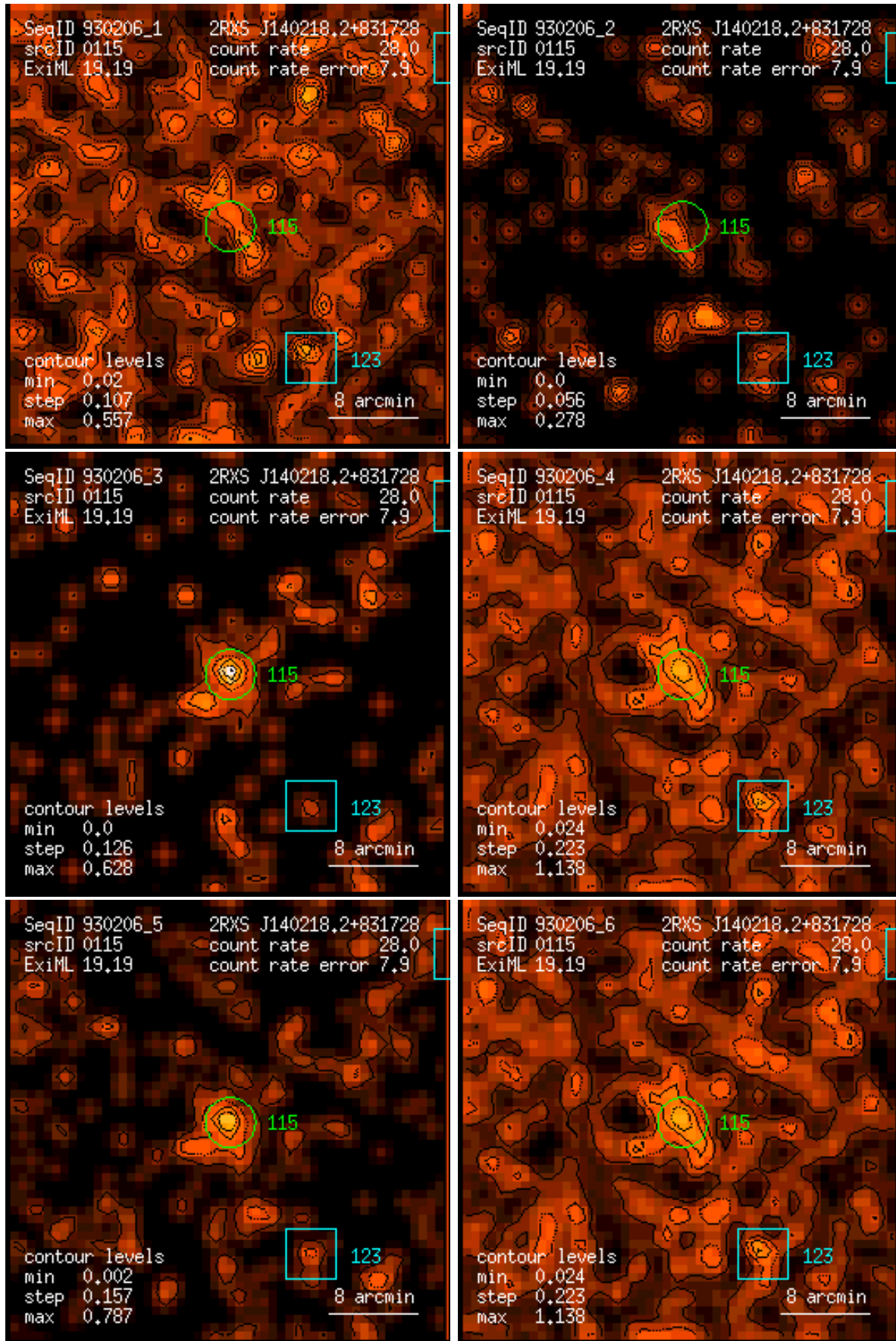
Figure 115: RASS 930206: detection 0115: band rate images, Gaussian filter: (1) PSPC channels 11 – 41, (2) 52 – 90, (3) 91 – 201, (4) 11 – 235, (5) 52 – 201, (6) 11 – 201. Broad band rates in counts/ks. Band rate contour levels in counts/ks/arcmin 2 .
