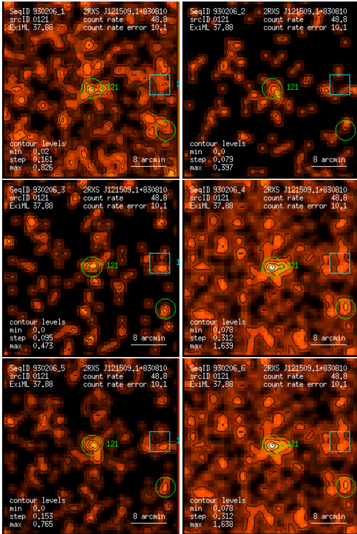
Figure 121: RASS 930206: detection 0121: band rate images, Gaussian filter: (1) PSPC channels 11 – 41, (2) 52 – 90, (3) 91 – 201, (4) 11 – 235, (5) 52 – 201, (6) 11 – 201. Broad band rates in counts/ks. Band rate contour levels in counts/ks/arcmin 2 .
