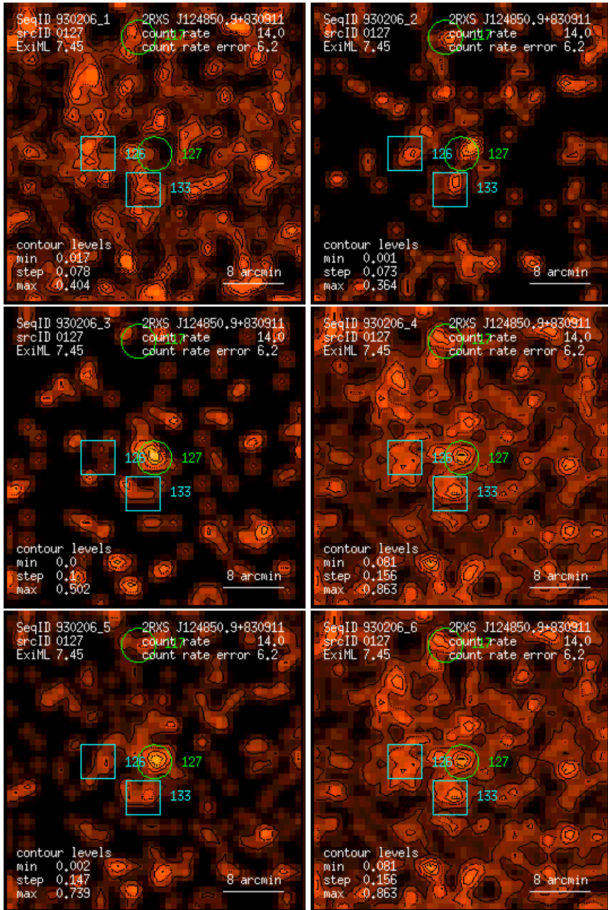
Figure 127: RASS 930206: detection 0127: band rate images, Gaussian filter: (1) PSPC channels 11 – 41, (2) 52 – 90, (3) 91 – 201, (4) 11 – 235, (5) 52 – 201, (6) 11 – 201. Broad band rates in counts/ks. Band rate contour levels in counts/ks/arcmin 2 .
