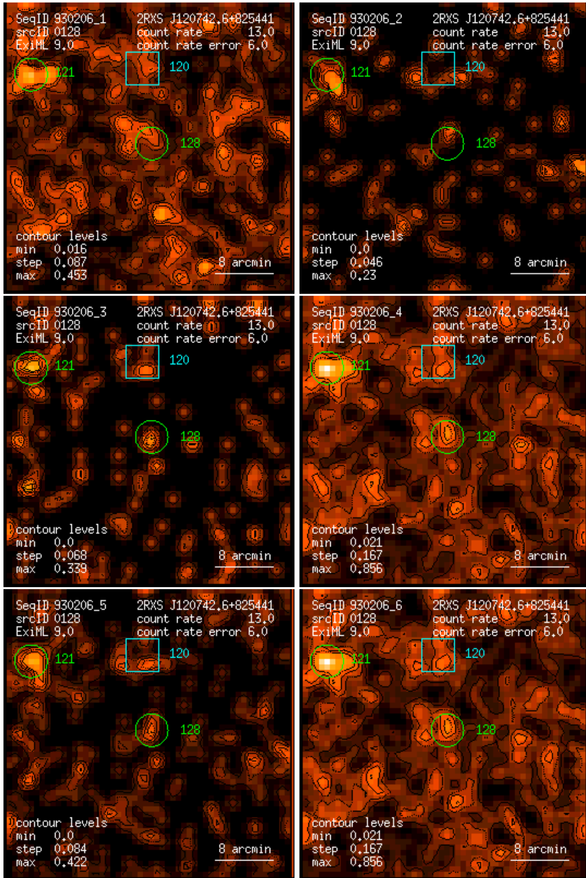
Figure 128: RASS 930206: detection 0128: band rate images, Gaussian filter: (1) PSPC channels 11 – 41, (2) 52 – 90, (3) 91 – 201, (4) 11 – 235, (5) 52 – 201, (6) 11 – 201. Broad band rates in counts/ks. Band rate contour levels in counts/ks/arcmin 2 .
