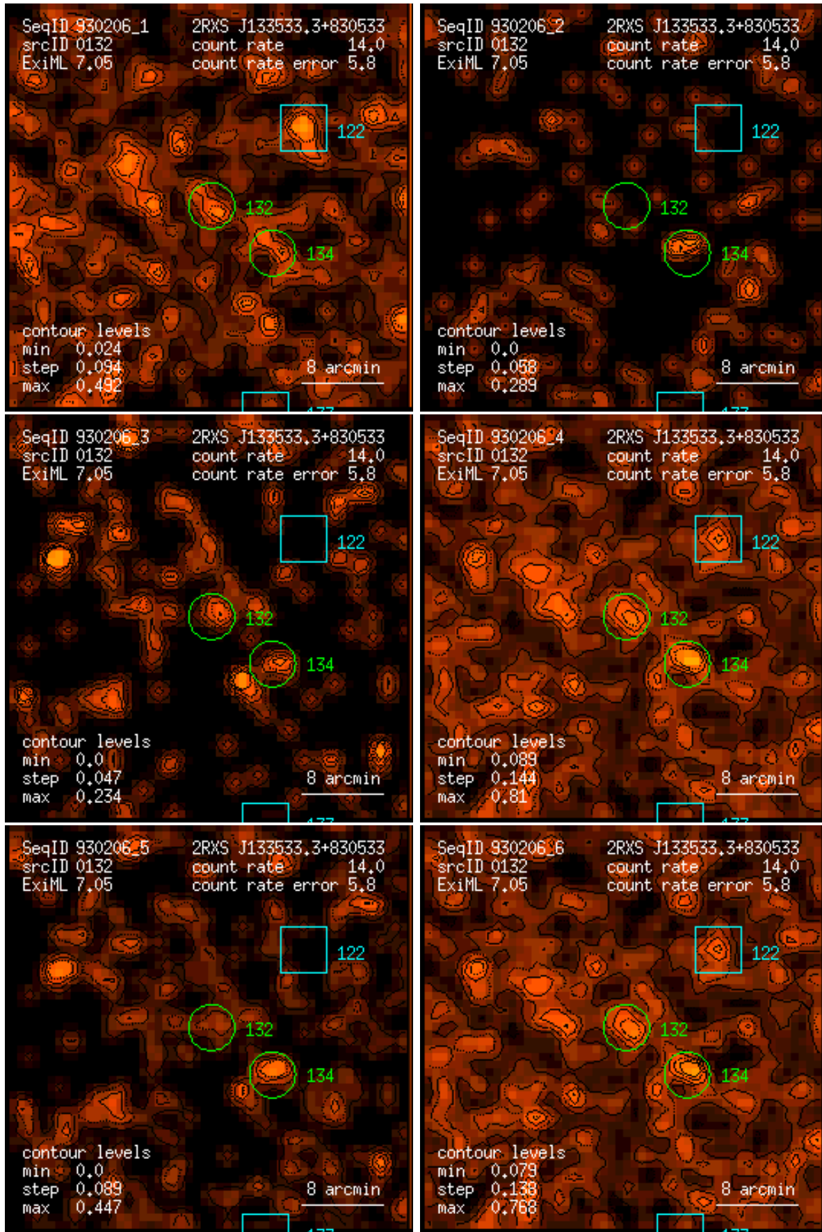
Figure 132: RASS 930206: detection 0132: band rate images, Gaussian filter: (1) PSPC channels 11 – 41, (2) 52 – 90, (3) 91 – 201, (4) 11 – 235, (5) 52 – 201, (6) 11 – 201. Broad band rates in counts/ks. Band rate contour levels in counts/ks/arcmin 2 .
