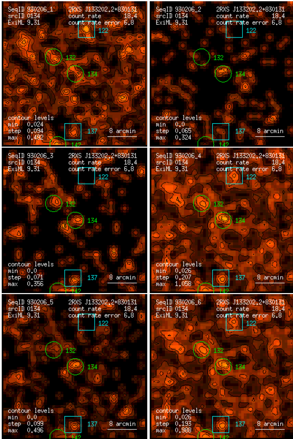
Figure 134: RASS 930206: detection 0134: band rate images, Gaussian filter: (1) PSPC channels 11 – 41, (2) 52 – 90, (3) 91 – 201, (4) 11 – 235, (5) 52 – 201, (6) 11 – 201. Broad band rates in counts/ks. Band rate contour levels in counts/ks/arcmin 2 .
