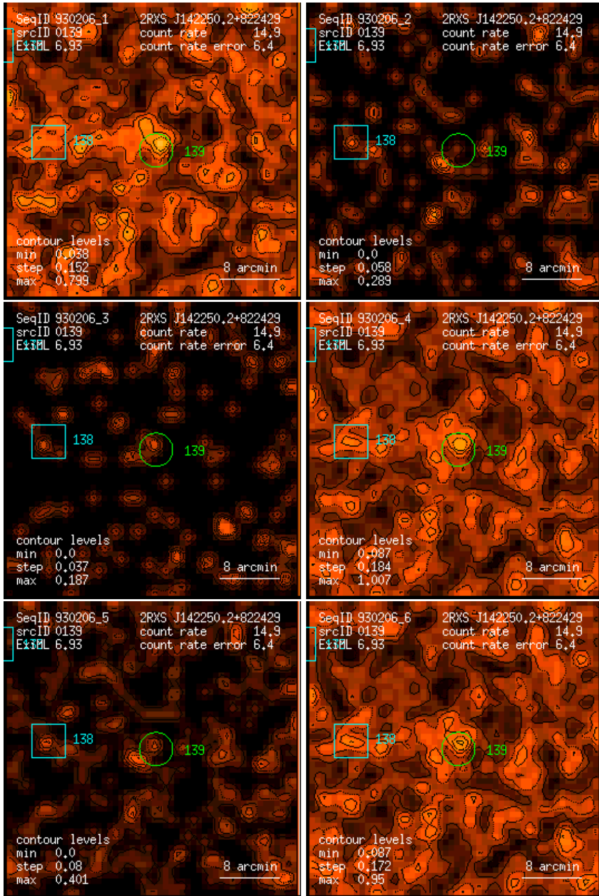
Figure 139: RASS 930206: detection 0139: band rate images, Gaussian filter: (1) PSPC channels 11 – 41, (2) 52 – 90, (3) 91 – 201, (4) 11 – 235, (5) 52 – 201, (6) 11 – 201. Broad band rates in counts/ks. Band rate contour levels in counts/ks/arcmin 2 .
