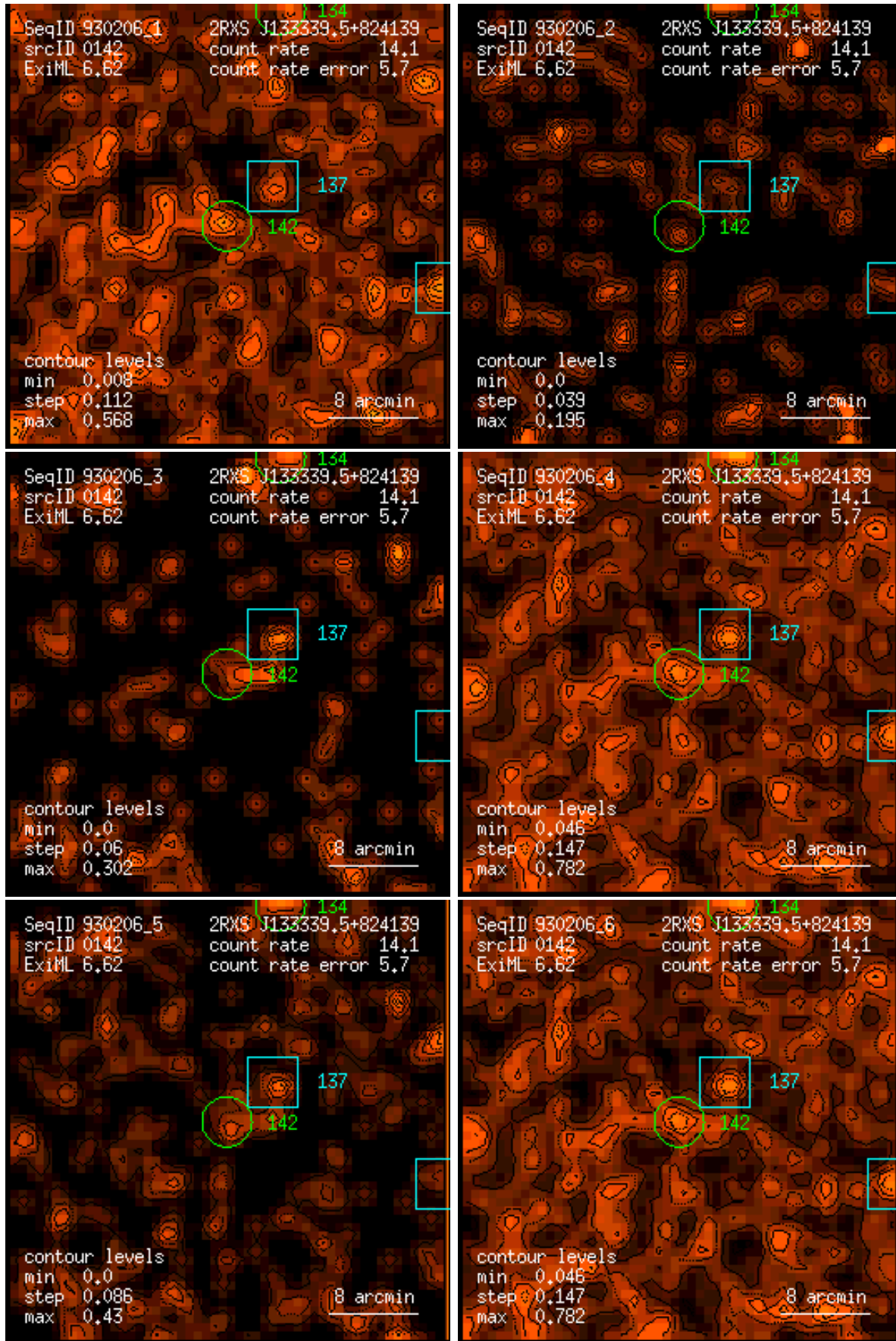
Figure 142: RASS 930206: detection 0142: band rate images, Gaussian filter: (1) PSPC channels 11 – 41, (2) 52 – 90, (3) 91 – 201, (4) 11 – 235, (5) 52 – 201, (6) 11 – 201. Broad band rates in counts/ks. Band rate contour levels in counts/ks/arcmin 2 .
