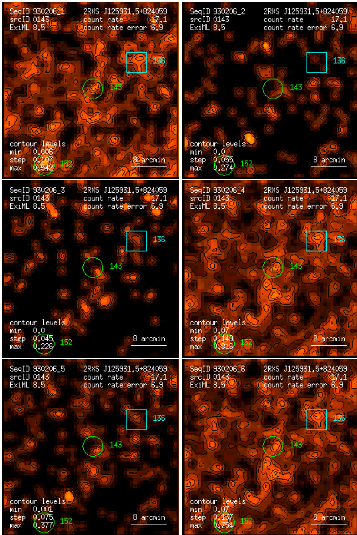
Figure 143: RASS 930206: detection 0143: band rate images, Gaussian filter: (1) PSPC channels 11 – 41, (2) 52 – 90, (3) 91 – 201, (4) 11 – 235, (5) 52 – 201, (6) 11 – 201. Broad band rates in counts/ks. Band rate contour levels in counts/ks/arcmin 2 .
