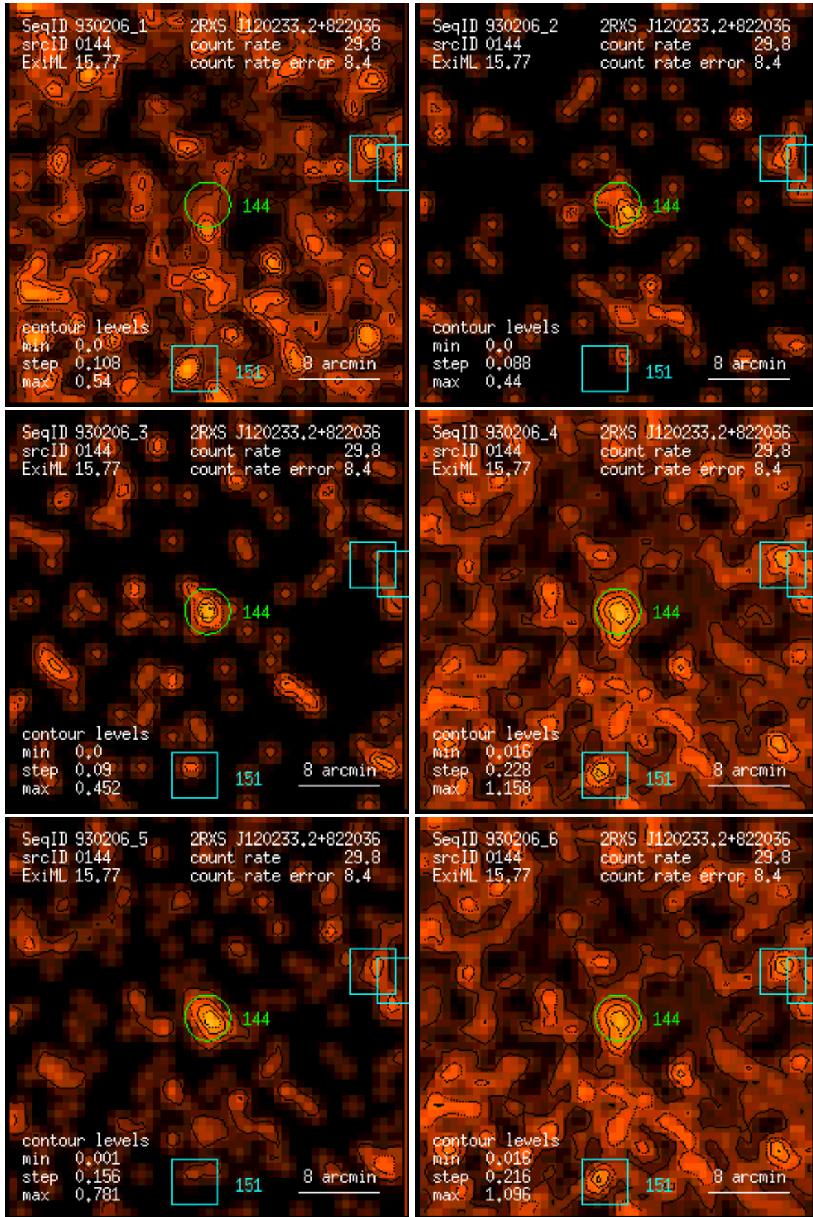
Figure 144: RASS 930206: detection 0144: band rate images, Gaussian filter: (1) PSPC channels 11 – 41, (2) 52 – 90, (3) 91 – 201, (4) 11 – 235, (5) 52 – 201, (6) 11 – 201. Broad band rates in counts/ks. Band rate contour levels in counts/ks/arcmin 2 .
