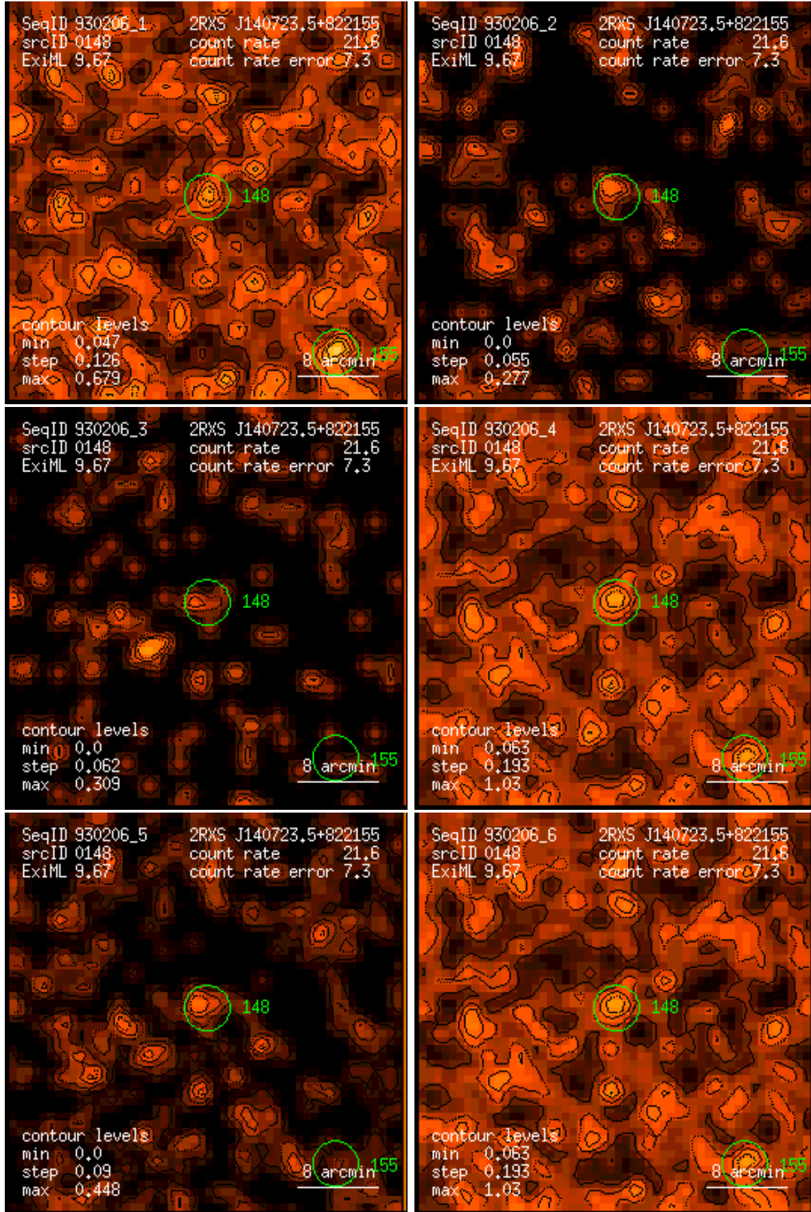
Figure 148: RASS 930206: detection 0148: band rate images, Gaussian filter: (1) PSPC channels 11 – 41, (2) 52 – 90, (3) 91 – 201, (4) 11 – 235, (5) 52 – 201, (6) 11 – 201. Broad band rates in counts/ks. Band rate contour levels in counts/ks/arcmin 2 .
