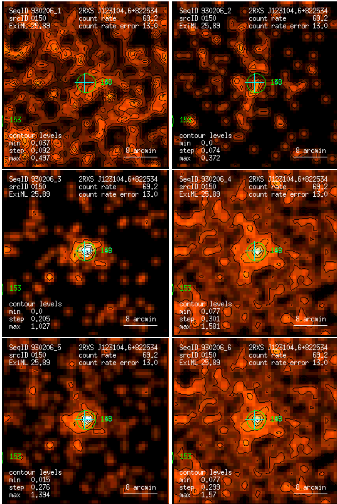
Figure 150: RASS 930206: detection 0150: band rate images, Gaussian filter: (1) PSPC channels 11 – 41, (2) 52 – 90, (3) 91 – 201, (4) 11 – 235, (5) 52 – 201, (6) 11 – 201. Broad band rates in counts/ks. Band rate contour levels in counts/ks/arcmin 2 .
