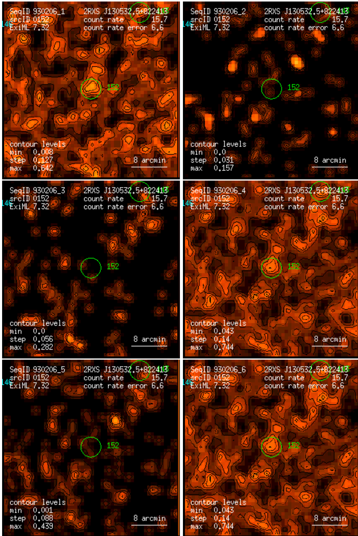
Figure 152: RASS 930206: detection 0152: band rate images, Gaussian filter: (1) PSPC channels 11 – 41, (2) 52 – 90, (3) 91 – 201, (4) 11 – 235, (5) 52 – 201, (6) 11 – 201. Broad band rates in counts/ks. Band rate contour levels in counts/ks/arcmin 2 .
