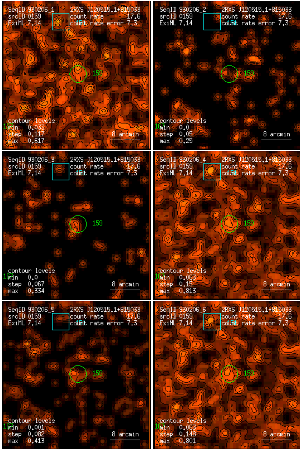
Figure 159: RASS 930206: detection 0159: band rate images, Gaussian filter: (1) PSPC channels 11 – 41, (2) 52 – 90, (3) 91 – 201, (4) 11 – 235, (5) 52 – 201, (6) 11 – 201. Broad band rates in counts/ks. Band rate contour levels in counts/ks/arcmin 2 .
