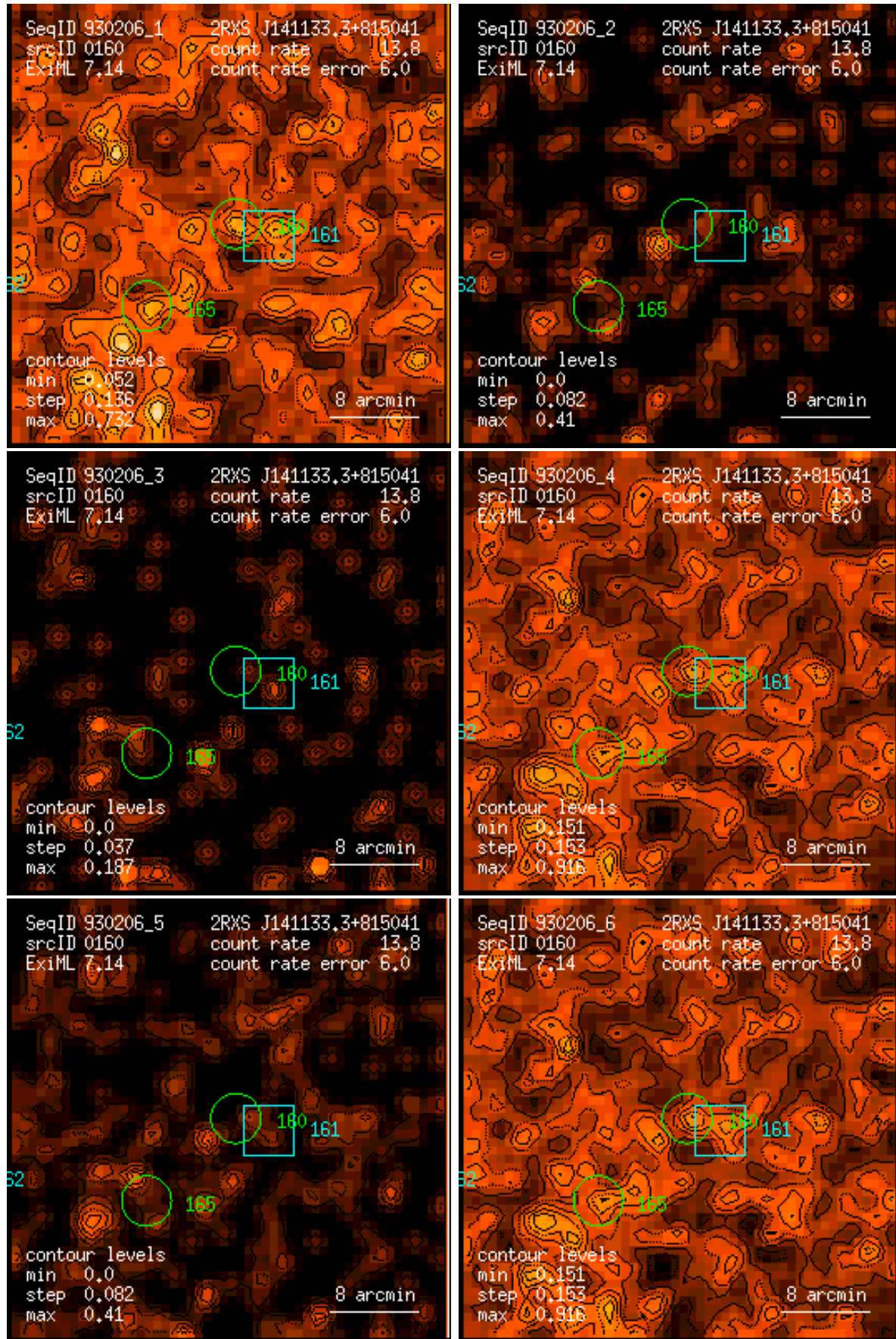
Figure 160: RASS 930206: detection 0160: band rate images, Gaussian filter: (1) PSPC channels 11 – 41, (2) 52 – 90, (3) 91 – 201, (4) 11 – 235, (5) 52 – 201, (6) 11 – 201. Broad band rates in counts/ks. Band rate contour levels in counts/ks/arcmin 2 .
