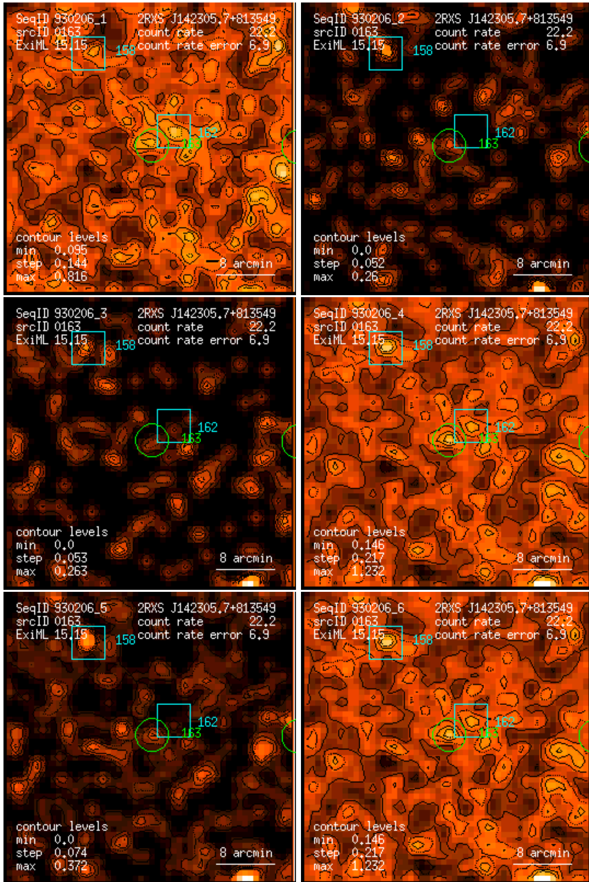
Figure 163: RASS 930206: detection 0163: band rate images, Gaussian filter: (1) PSPC channels 11 – 41, (2) 52 – 90, (3) 91 – 201, (4) 11 – 235, (5) 52 – 201, (6) 11 – 201. Broad band rates in counts/ks. Band rate contour levels in counts/ks/arcmin 2 .
