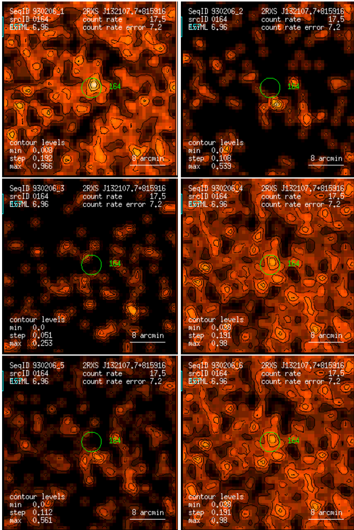
Figure 164: RASS 930206: detection 0164: band rate images, Gaussian filter: (1) PSPC channels 11 – 41, (2) 52 – 90, (3) 91 – 201, (4) 11 – 235, (5) 52 – 201, (6) 11 – 201. Broad band rates in counts/ks. Band rate contour levels in counts/ks/arcmin 2 .
