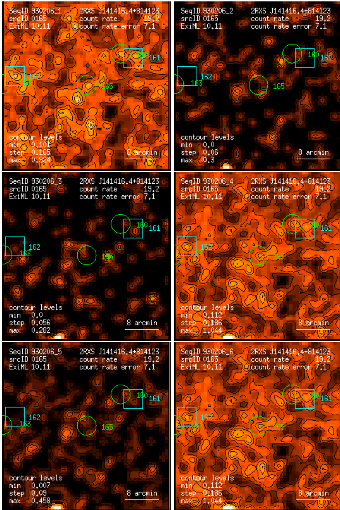
Figure 165: RASS 930206: detection 0165: band rate images, Gaussian filter: (1) PSPC channels 11 – 41, (2) 52 – 90, (3) 91 – 201, (4) 11 – 235, (5) 52 – 201, (6) 11 – 201. Broad band rates in counts/ks. Band rate contour levels in counts/ks/arcmin 2 .
