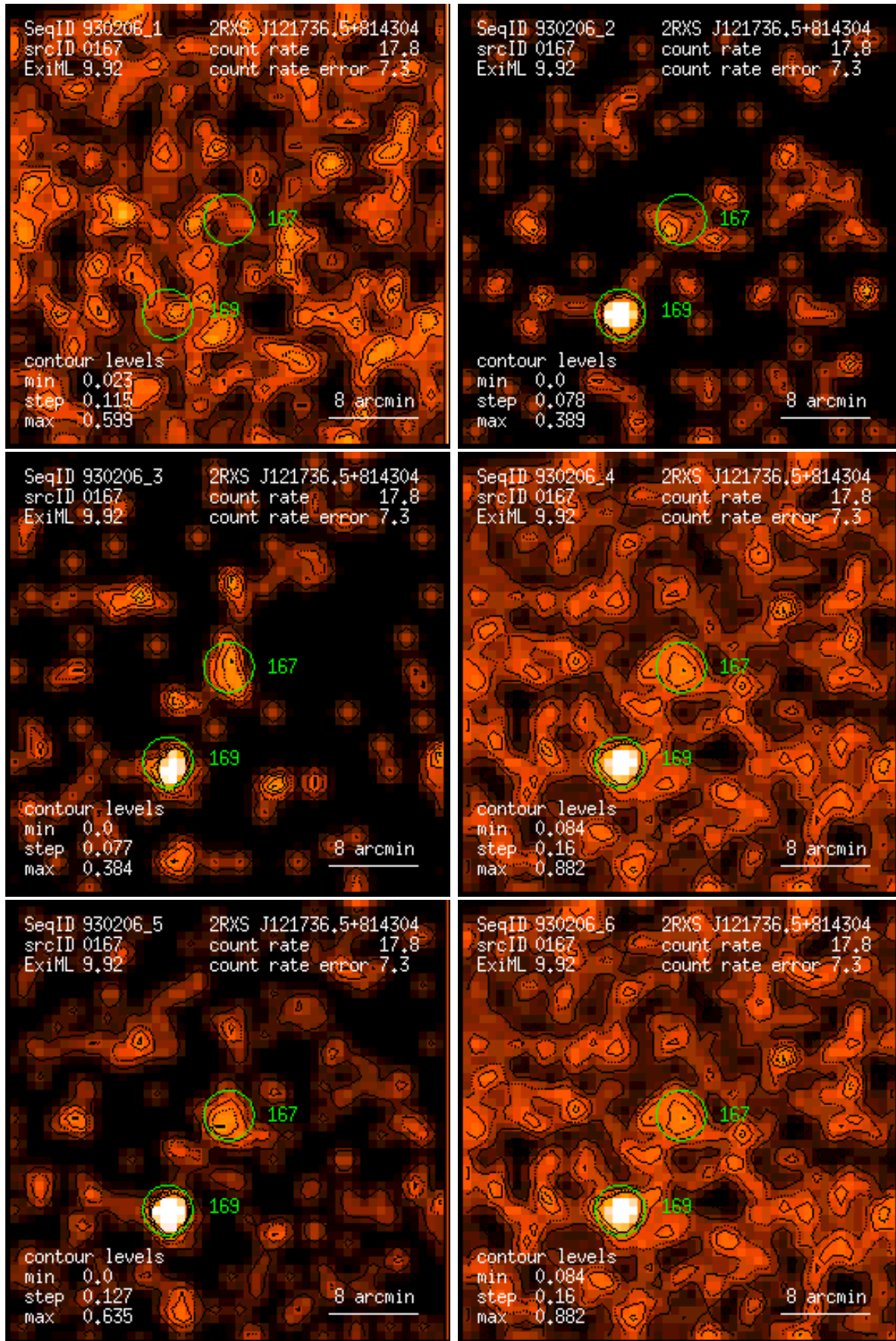
Figure 167: RASS 930206: detection 0167: band rate images, Gaussian filter: (1) PSPC channels 11 – 41, (2) 52 – 90, (3) 91 – 201, (4) 11 – 235, (5) 52 – 201, (6) 11 – 201. Broad band rates in counts/ks. Band rate contour levels in counts/ks/arcmin 2 .
