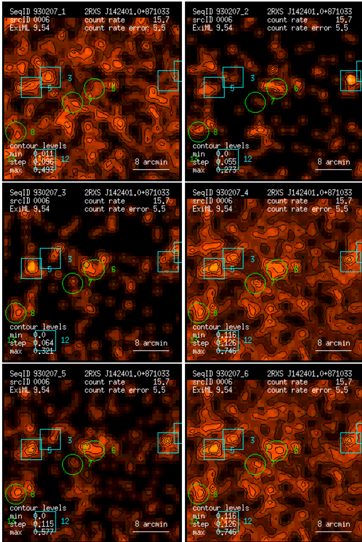
Figure 6: RASS 930207: detection 0006: band rate images, Gaussian filter: (1) PSPC channels 11 – 41, (2) 52 – 90, (3) 91 – 201, (4) 11 – 235, (5) 52 – 201, (6) 11 – 201. Broad band rates in counts/ks. Band rate contour levels in counts/ks/arcmin 2 .
