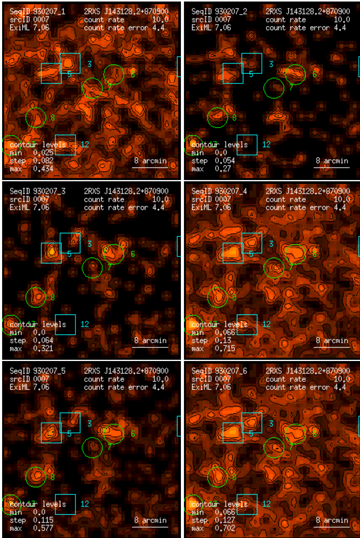
Figure 7: RASS 930207: detection 0007: band rate images, Gaussian filter: (1) PSPC channels 11 – 41, (2) 52 – 90, (3) 91 – 201, (4) 11 – 235, (5) 52 – 201, (6) 11 – 201. Broad band rates in counts/ks. Band rate contour levels in counts/ks/arcmin 2 .
