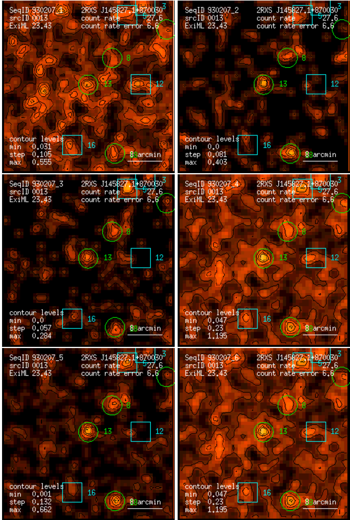
Figure 13: RASS 930207: detection 0013: band rate images, Gaussian filter: (1) PSPC channels 11 – 41, (2) 52 – 90, (3) 91 – 201, (4) 11 – 235, (5) 52 – 201, (6) 11 – 201. Broad band rates in counts/ks. Band rate contour levels in counts/ks/arcmin 2 .
