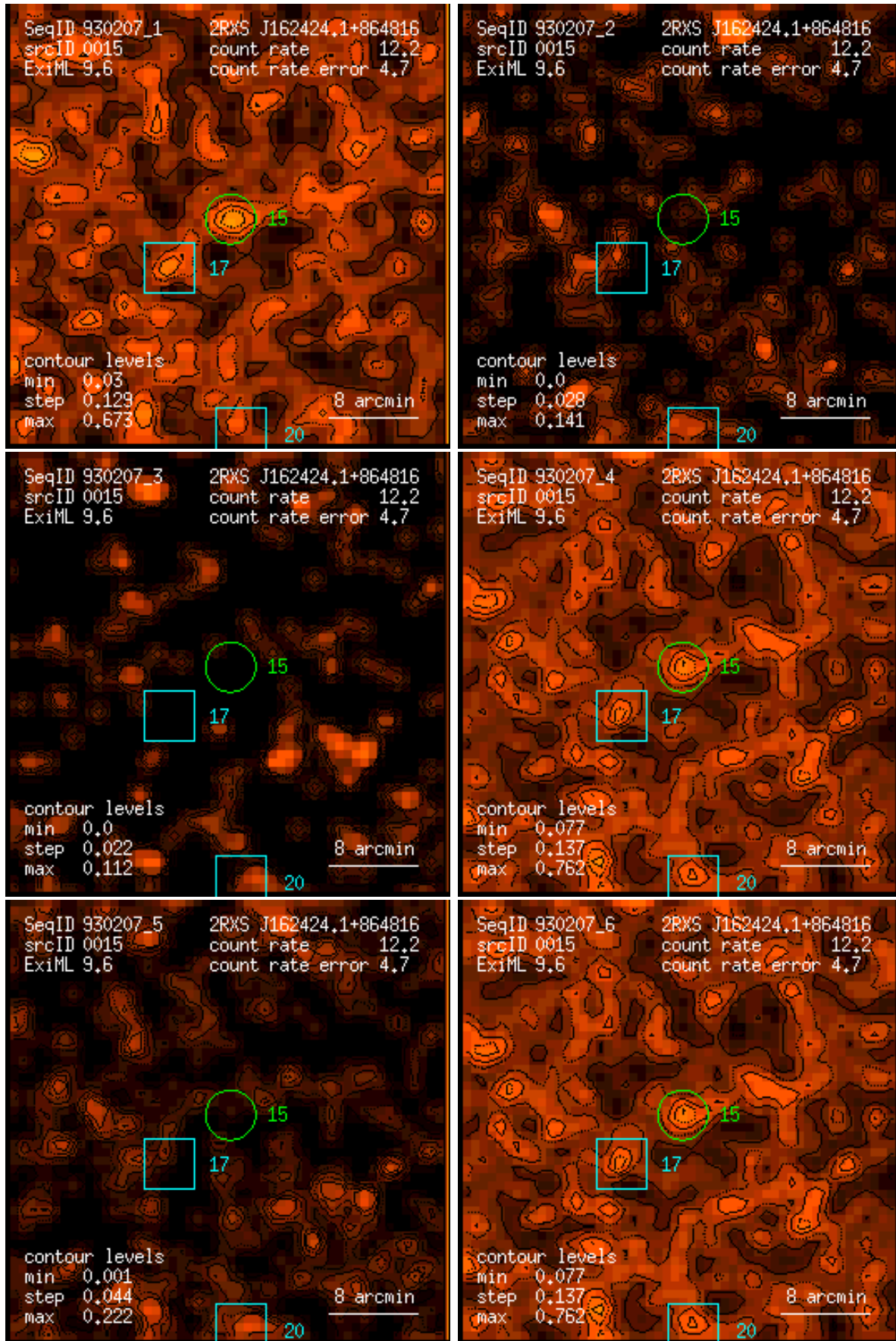
Figure 15: RASS 930207: detection 0015: band rate images, Gaussian filter: (1) PSPC channels 11 – 41, (2) 52 – 90, (3) 91 – 201, (4) 11 – 235, (5) 52 – 201, (6) 11 – 201. Broad band rates in counts/ks. Band rate contour levels in counts/ks/arcmin 2 .
