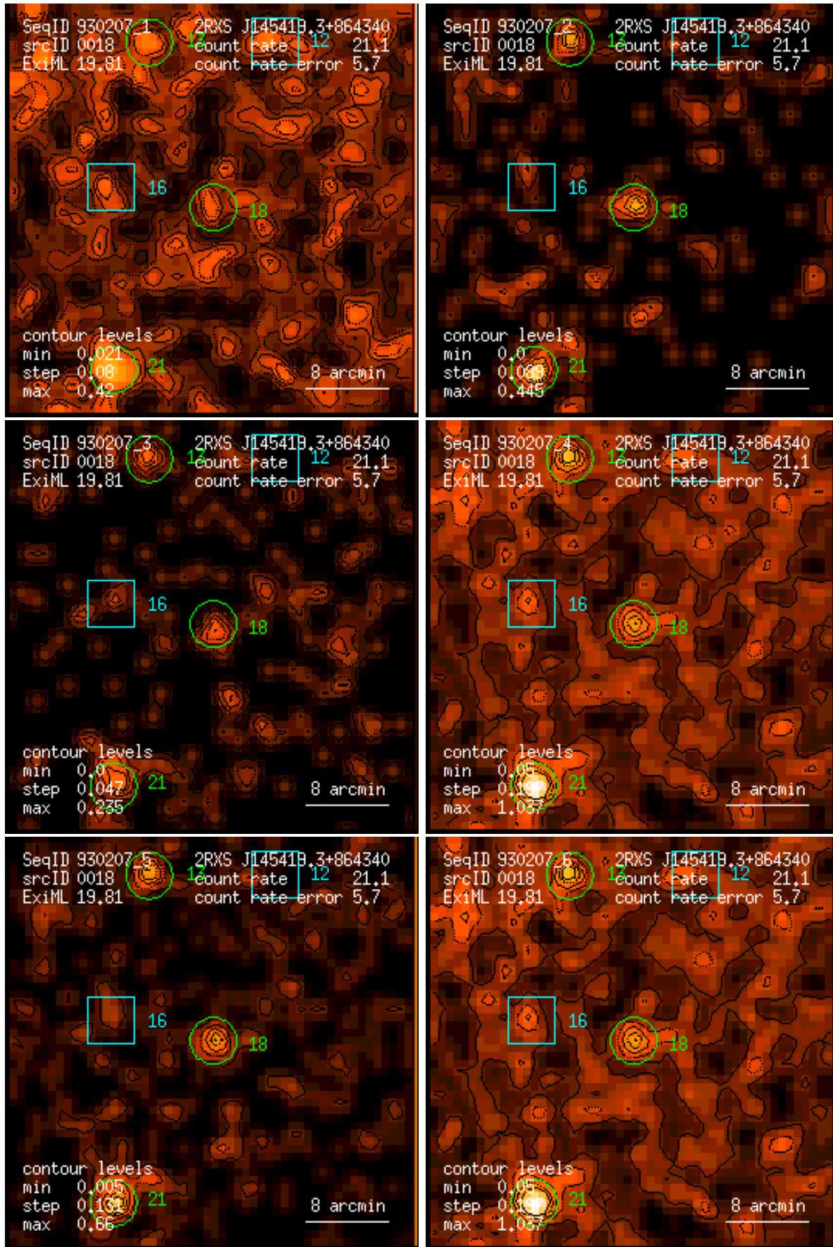
Figure 18: RASS 930207: detection 0018: band rate images, Gaussian filter: (1) PSPC channels 11 – 41, (2) 52 – 90, (3) 91 – 201, (4) 11 – 235, (5) 52 – 201, (6) 11 – 201. Broad band rates in counts/ks. Band rate contour levels in counts/ks/arcmin 2 .
