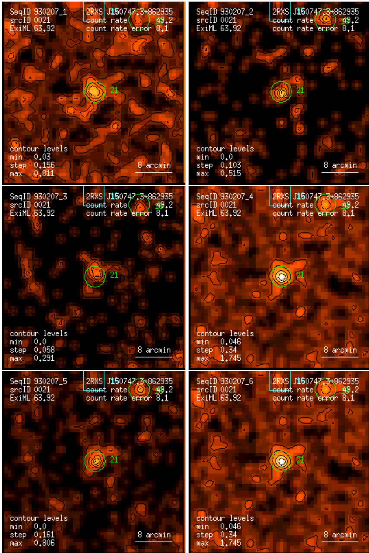
Figure 21: RASS 930207: detection 0021: band rate images, Gaussian filter: (1) PSPC channels 11 – 41, (2) 52 – 90, (3) 91 – 201, (4) 11 – 235, (5) 52 – 201, (6) 11 – 201. Broad band rates in counts/ks. Band rate contour levels in counts/ks/arcmin 2 .
