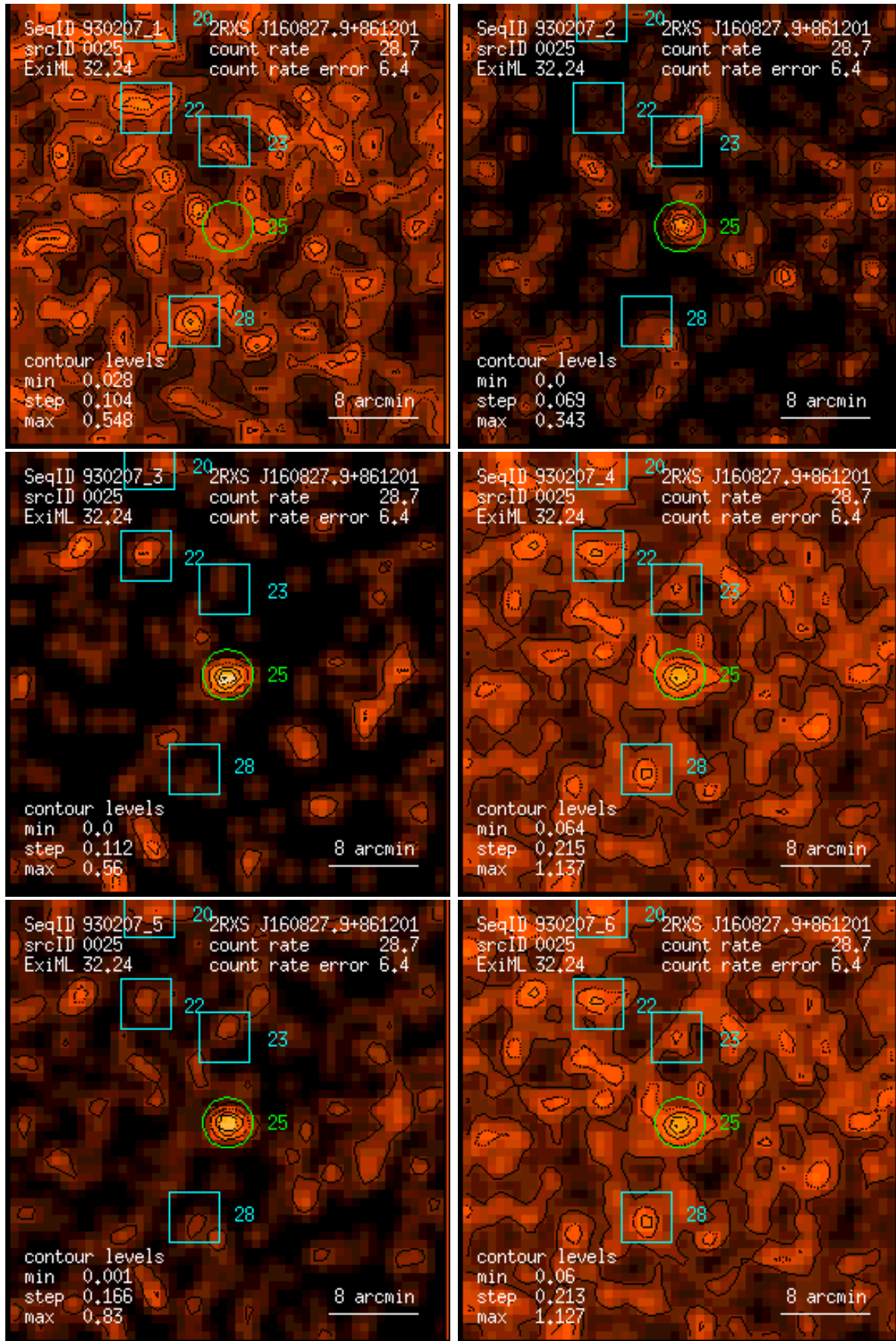
Figure 25: RASS 930207: detection 0025: band rate images, Gaussian filter: (1) PSPC channels 11 – 41, (2) 52 – 90, (3) 91 – 201, (4) 11 – 235, (5) 52 – 201, (6) 11 – 201. Broad band rates in counts/ks. Band rate contour levels in counts/ks/arcmin 2 .
