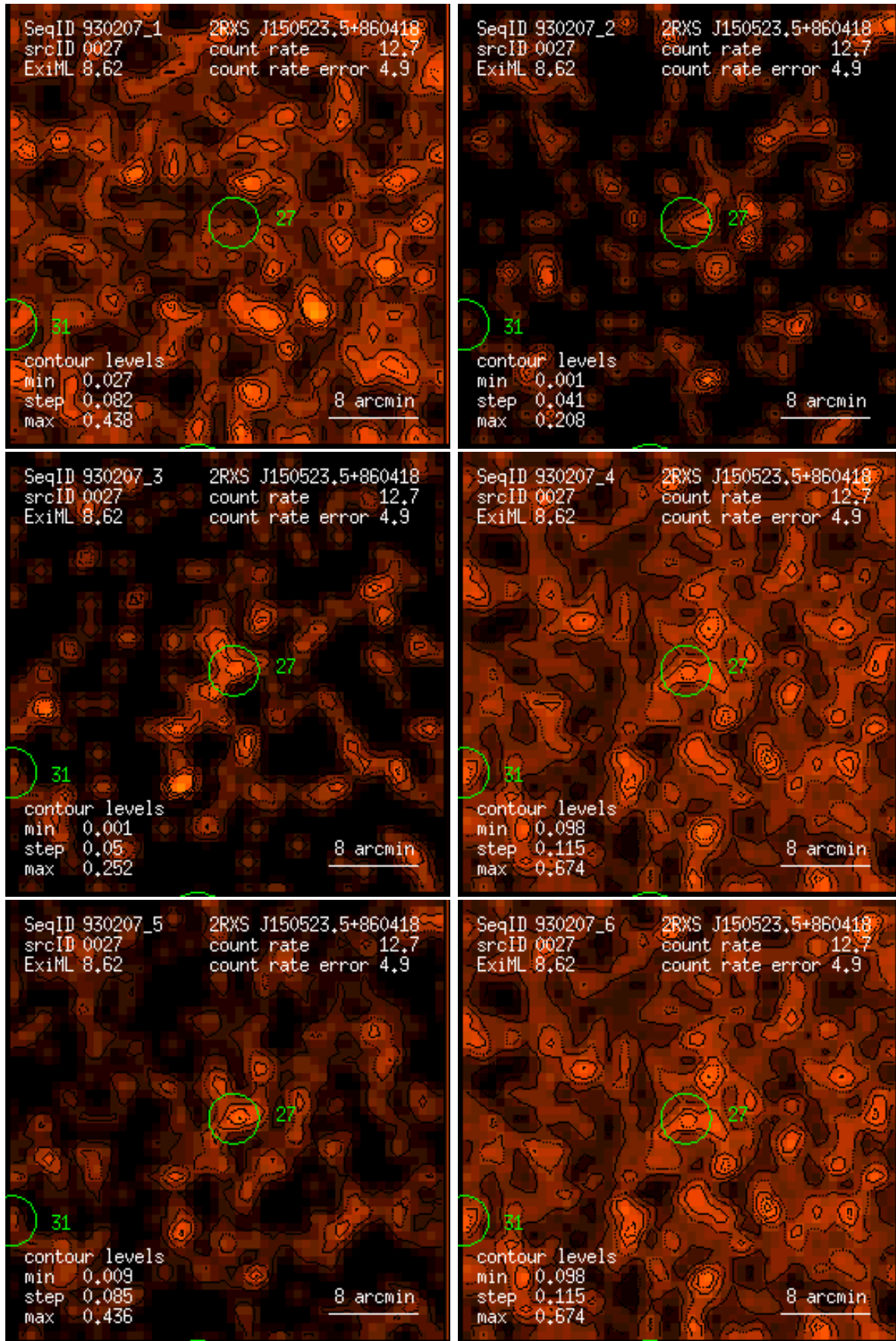
Figure 27: RASS 930207: detection 0027: band rate images, Gaussian filter: (1) PSPC channels 11 – 41, (2) 52 – 90, (3) 91 – 201, (4) 11 – 235, (5) 52 – 201, (6) 11 – 201. Broad band rates in counts/ks. Band rate contour levels in counts/ks/arcmin 2 .
