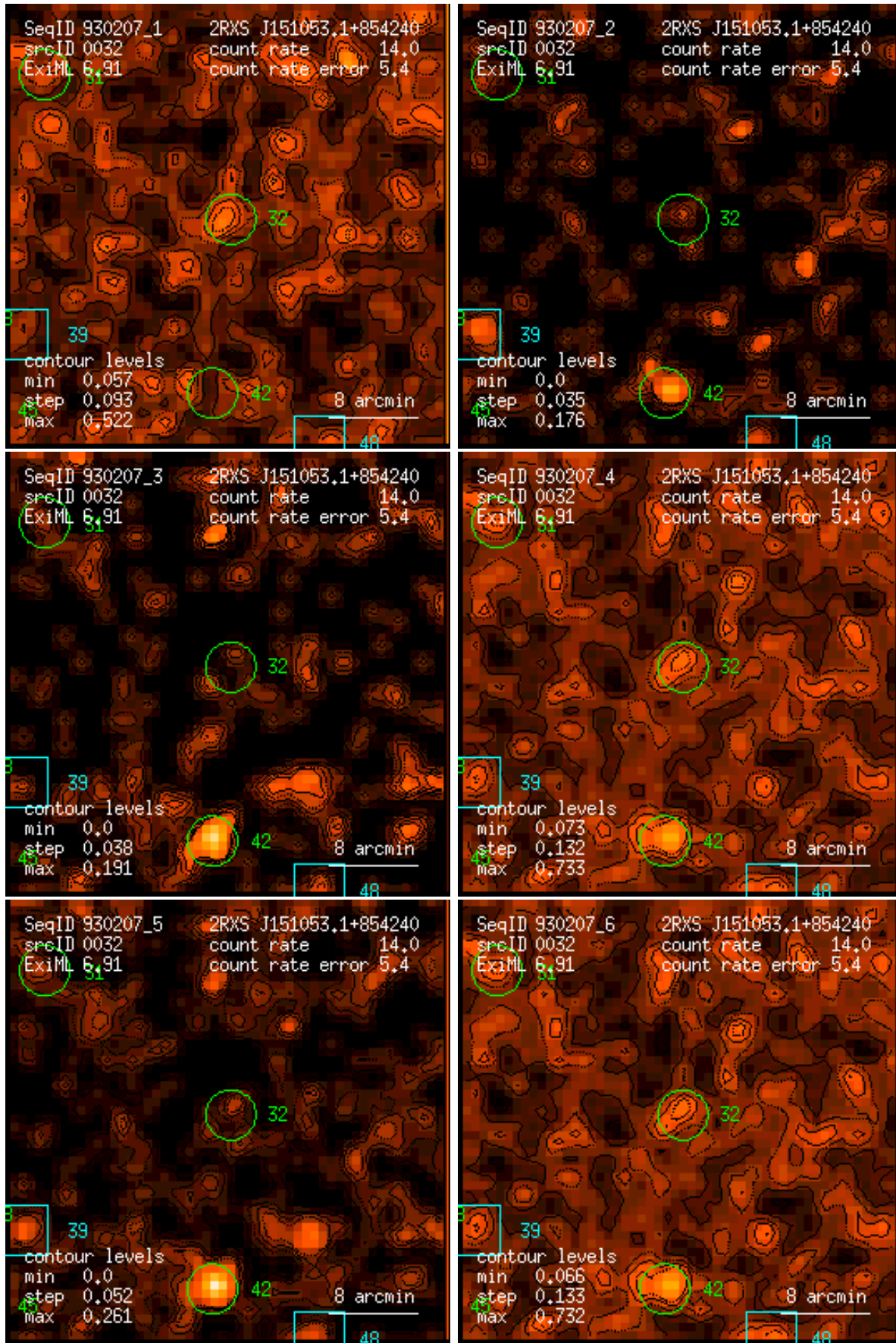
Figure 32: RASS 930207: detection 0032: band rate images, Gaussian filter: (1) PSPC channels 11 – 41, (2) 52 – 90, (3) 91 – 201, (4) 11 – 235, (5) 52 – 201, (6) 11 – 201. Broad band rates in counts/ks. Band rate contour levels in counts/ks/arcmin 2 .
