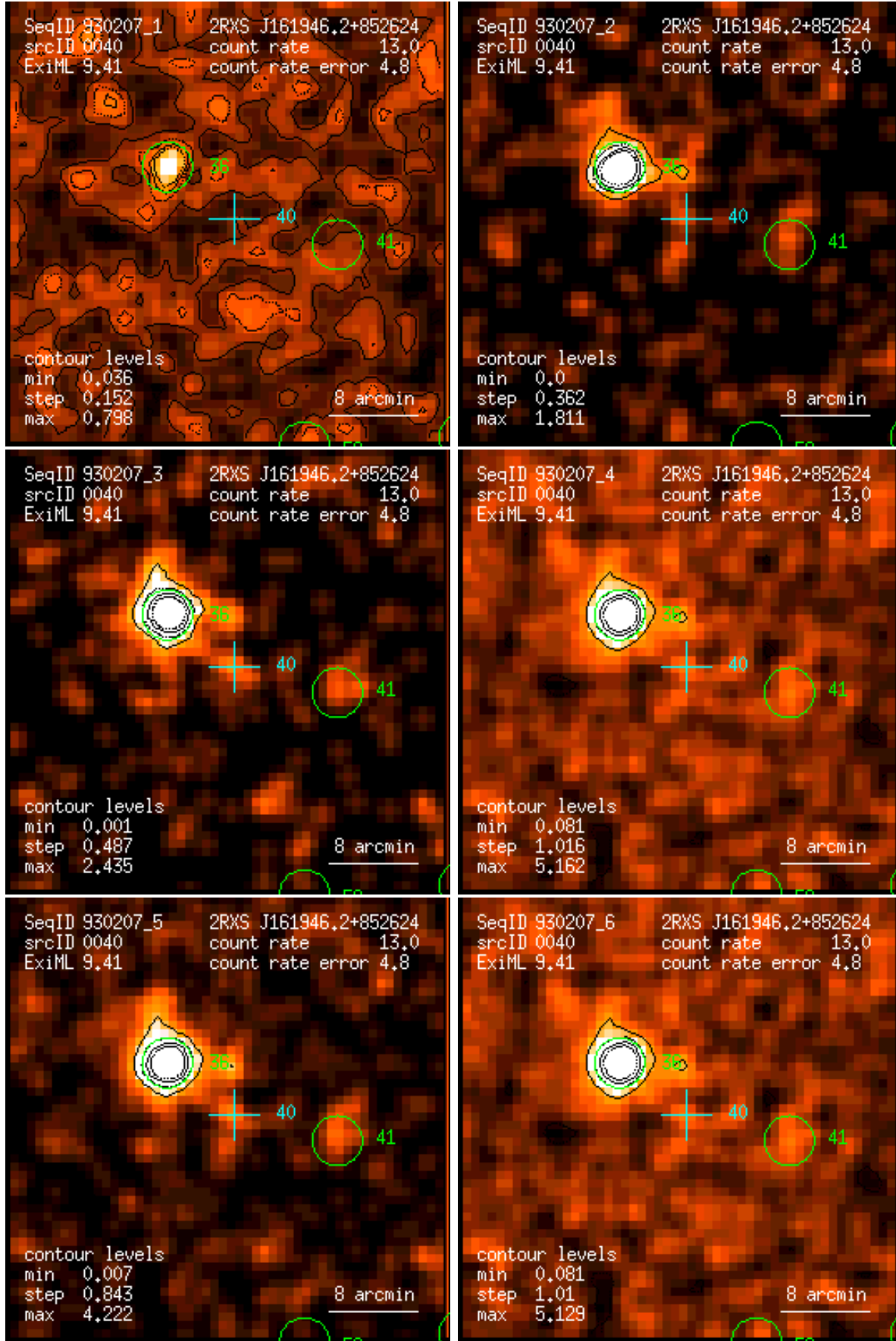
Figure 40: RASS 930207: detection 0040: band rate images, Gaussian filter: (1) PSPC channels 11 – 41, (2) 52 – 90, (3) 91 – 201, (4) 11 – 235, (5) 52 – 201, (6) 11 – 201. Broad band rates in counts/ks. Band rate contour levels in counts/ks/arcmin 2 .
