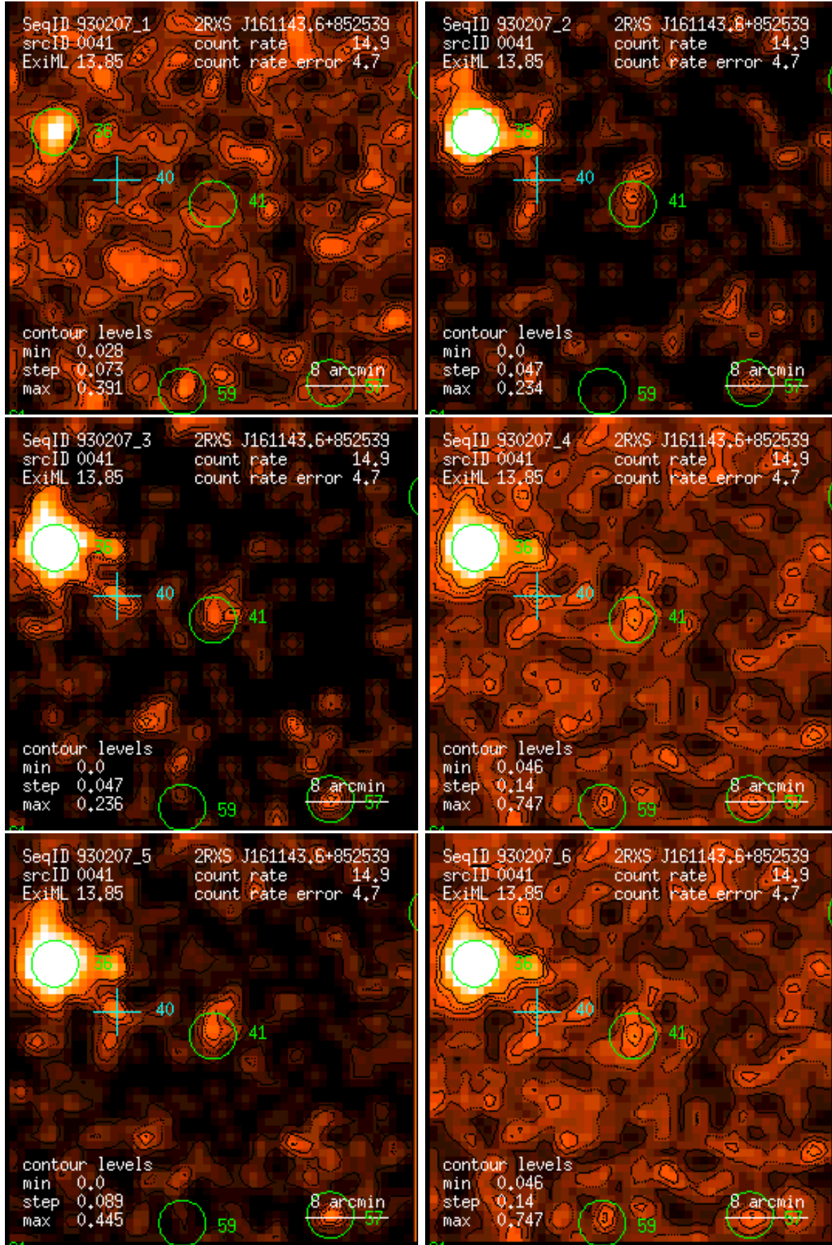
Figure 41: RASS 930207: detection 0041: band rate images, Gaussian filter: (1) PSPC channels 11 – 41, (2) 52 – 90, (3) 91 – 201, (4) 11 – 235, (5) 52 – 201, (6) 11 – 201. Broad band rates in counts/ks. Band rate contour levels in counts/ks/arcmin 2 .
