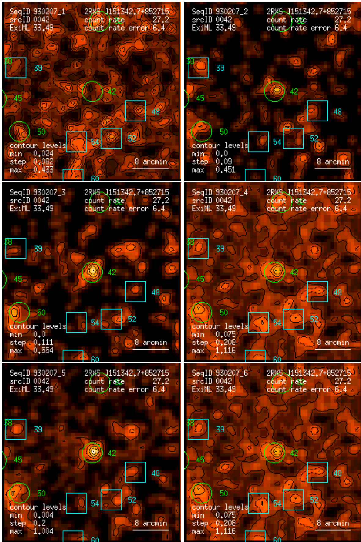
Figure 42: RASS 930207: detection 0042: band rate images, Gaussian filter: (1) PSPC channels 11 – 41, (2) 52 – 90, (3) 91 – 201, (4) 11 – 235, (5) 52 – 201, (6) 11 – 201. Broad band rates in counts/ks. Band rate contour levels in counts/ks/arcmin 2 .
