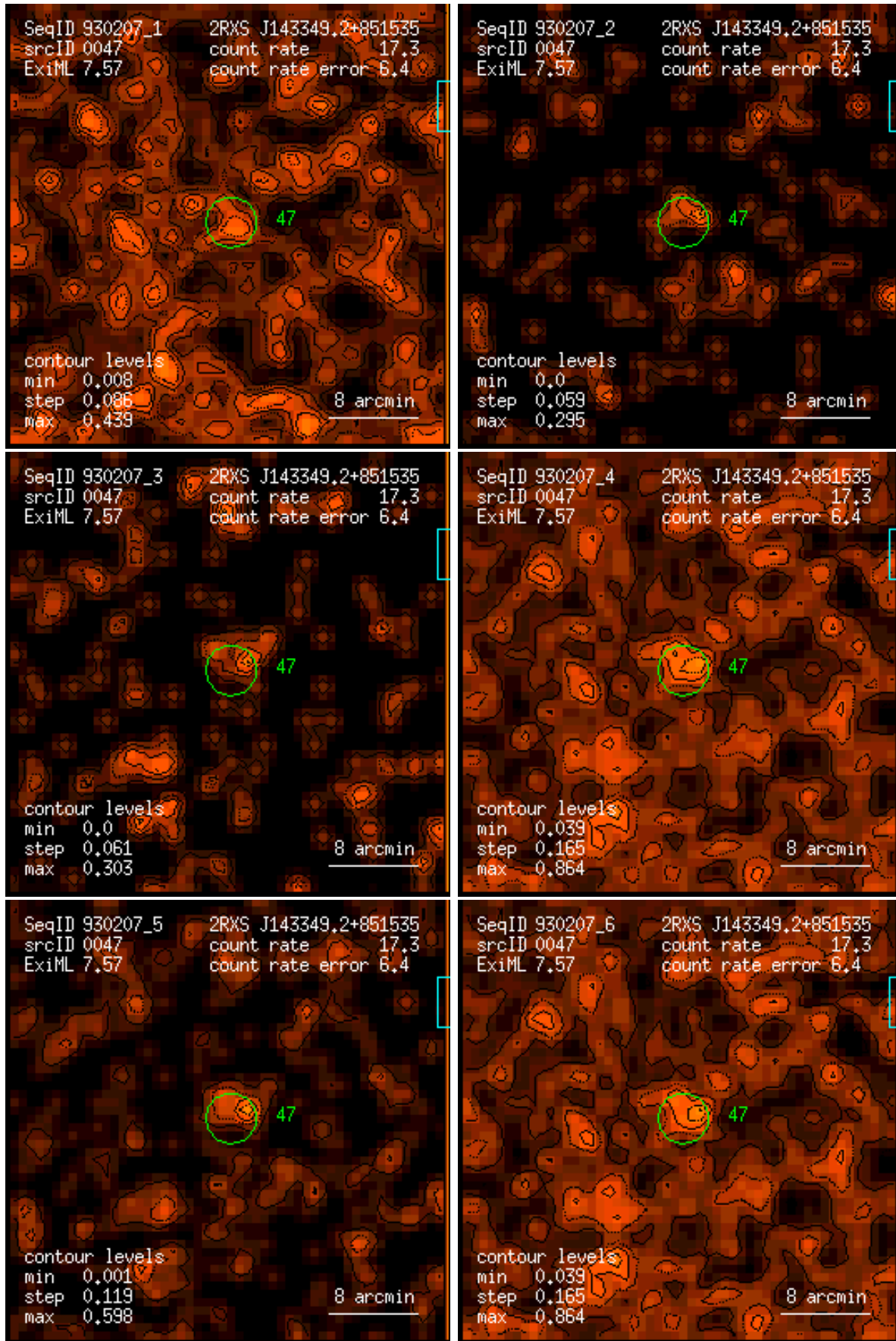
Figure 47: RASS 930207: detection 0047: band rate images, Gaussian filter: (1) PSPC channels 11 – 41, (2) 52 – 90, (3) 91 – 201, (4) 11 – 235, (5) 52 – 201, (6) 11 – 201. Broad band rates in counts/ks. Band rate contour levels in counts/ks/arcmin 2 .
