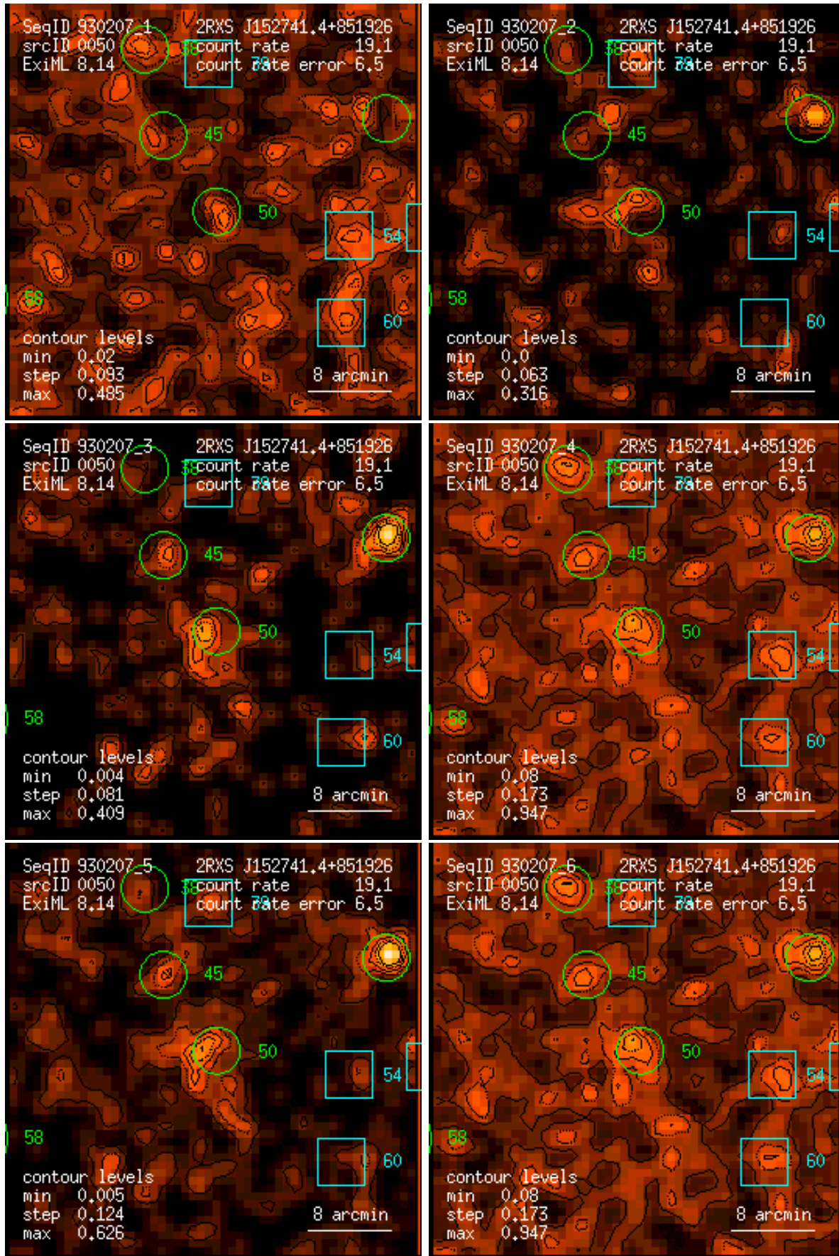
Figure 50: RASS 930207: detection 0050: band rate images, Gaussian filter: (1) PSPC channels 11 – 41, (2) 52 – 90, (3) 91 – 201, (4) 11 – 235, (5) 52 – 201, (6) 11 – 201. Broad band rates in counts/ks. Band rate contour levels in counts/ks/arcmin 2 .
