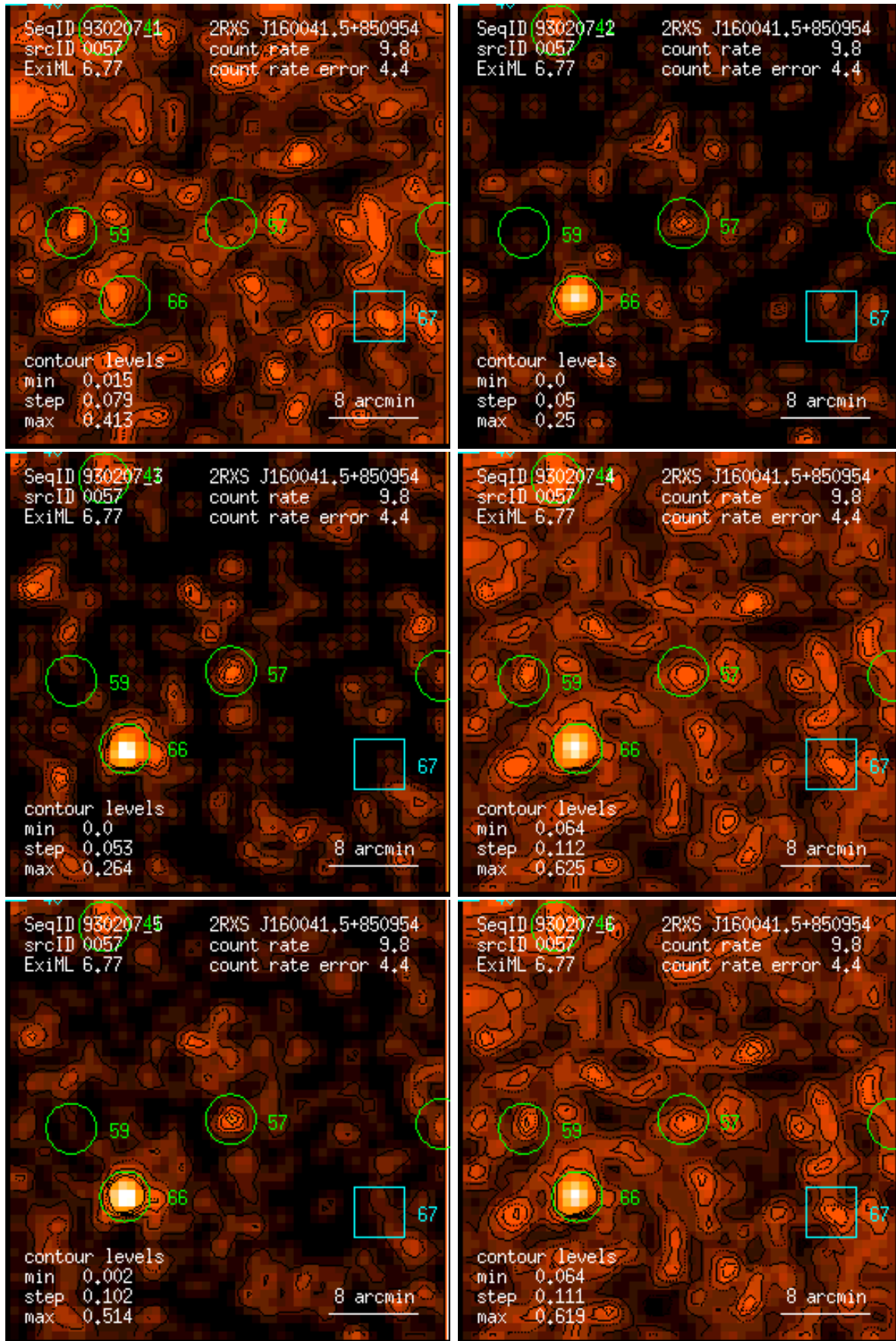
Figure 57: RASS 930207: detection 0057: band rate images, Gaussian filter: (1) PSPC channels 11 – 41, (2) 52 – 90, (3) 91 – 201, (4) 11 – 235, (5) 52 – 201, (6) 11 – 201. Broad band rates in counts/ks. Band rate contour levels in counts/ks/arcmin 2 .
