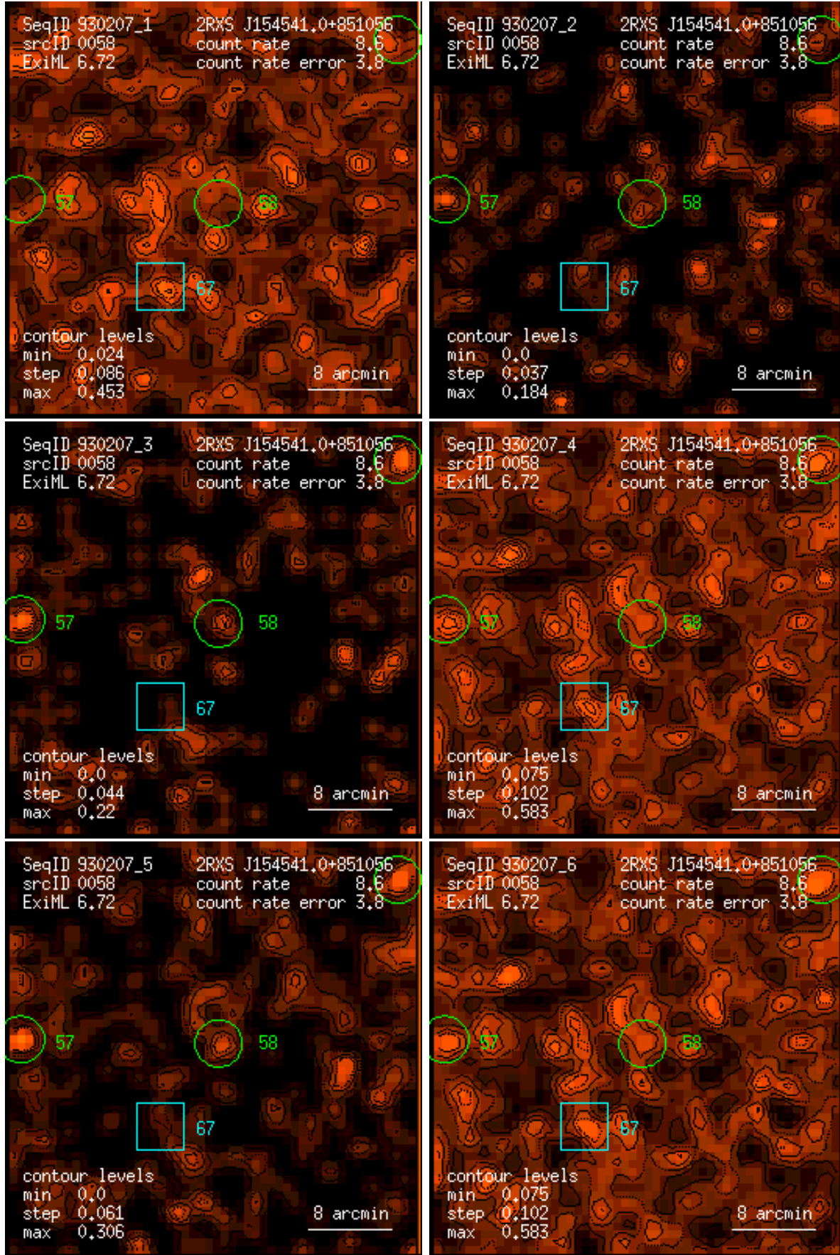
Figure 58: RASS 930207: detection 0058: band rate images, Gaussian filter: (1) PSPC channels 11 – 41, (2) 52 – 90, (3) 91 – 201, (4) 11 – 235, (5) 52 – 201, (6) 11 – 201. Broad band rates in counts/ks. Band rate contour levels in counts/ks/arcmin 2 .
